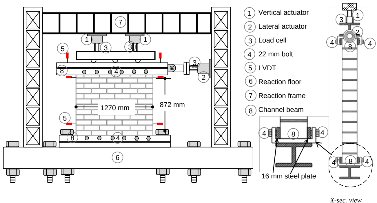
Fig. 6. Schematic diagram of experimental setup of shear wall
