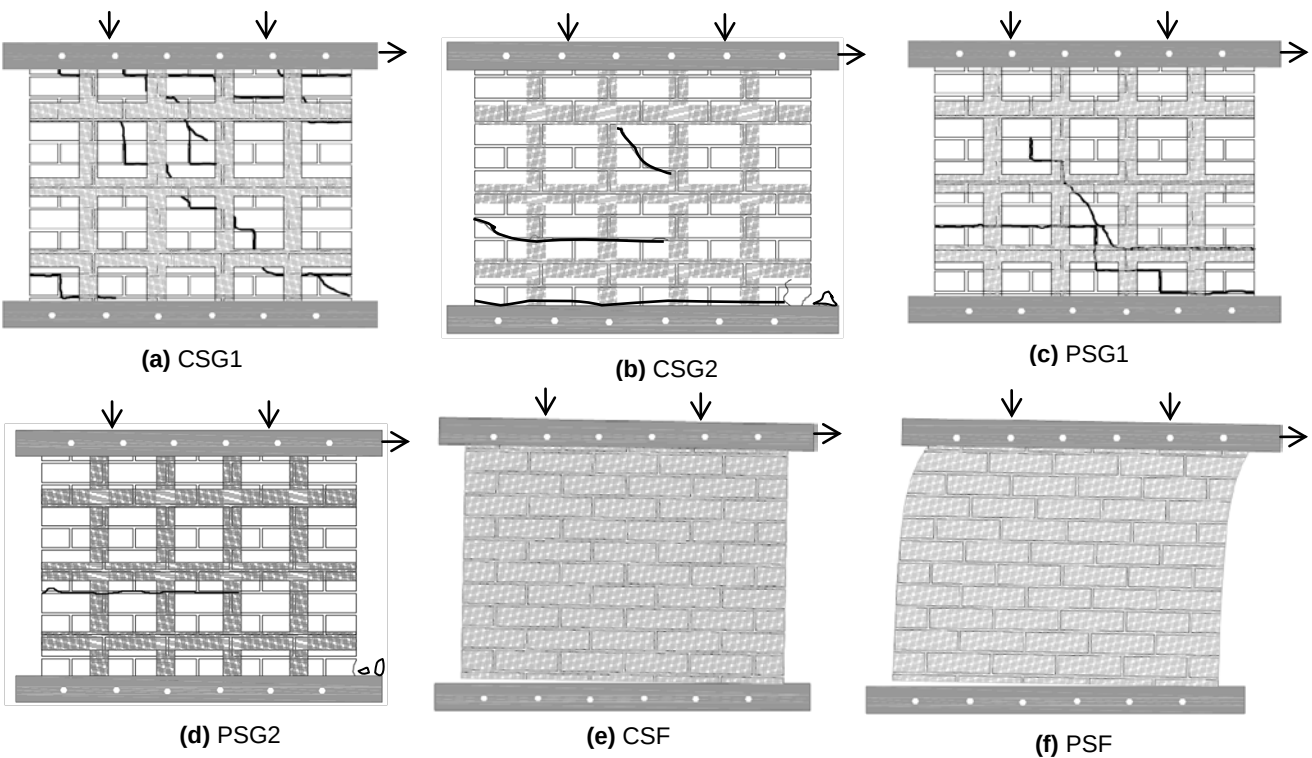
Fig. 11. Schematic representation of crack patterns in grid system and fully wrapped panels
