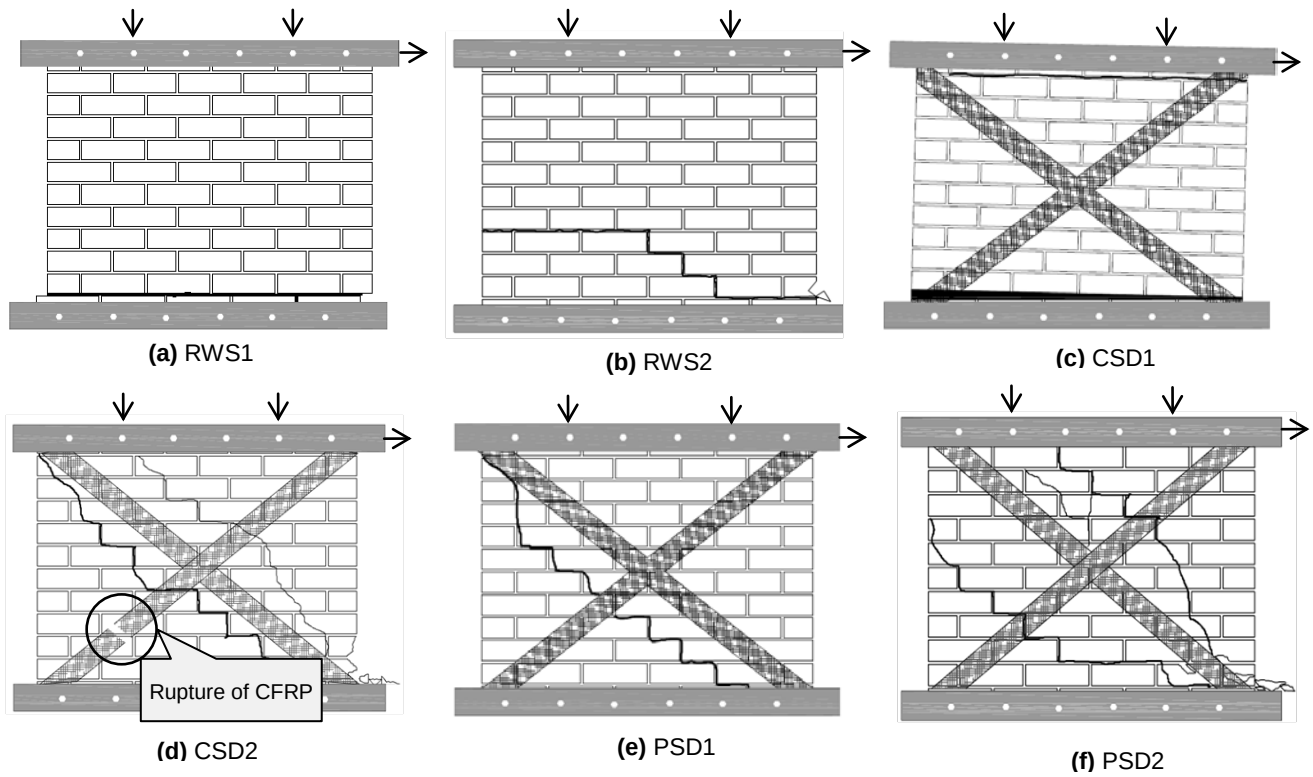
Fig. 10. Schematic illustration of crack patterns in unreinforced and FRP retrofitted masonry panels
