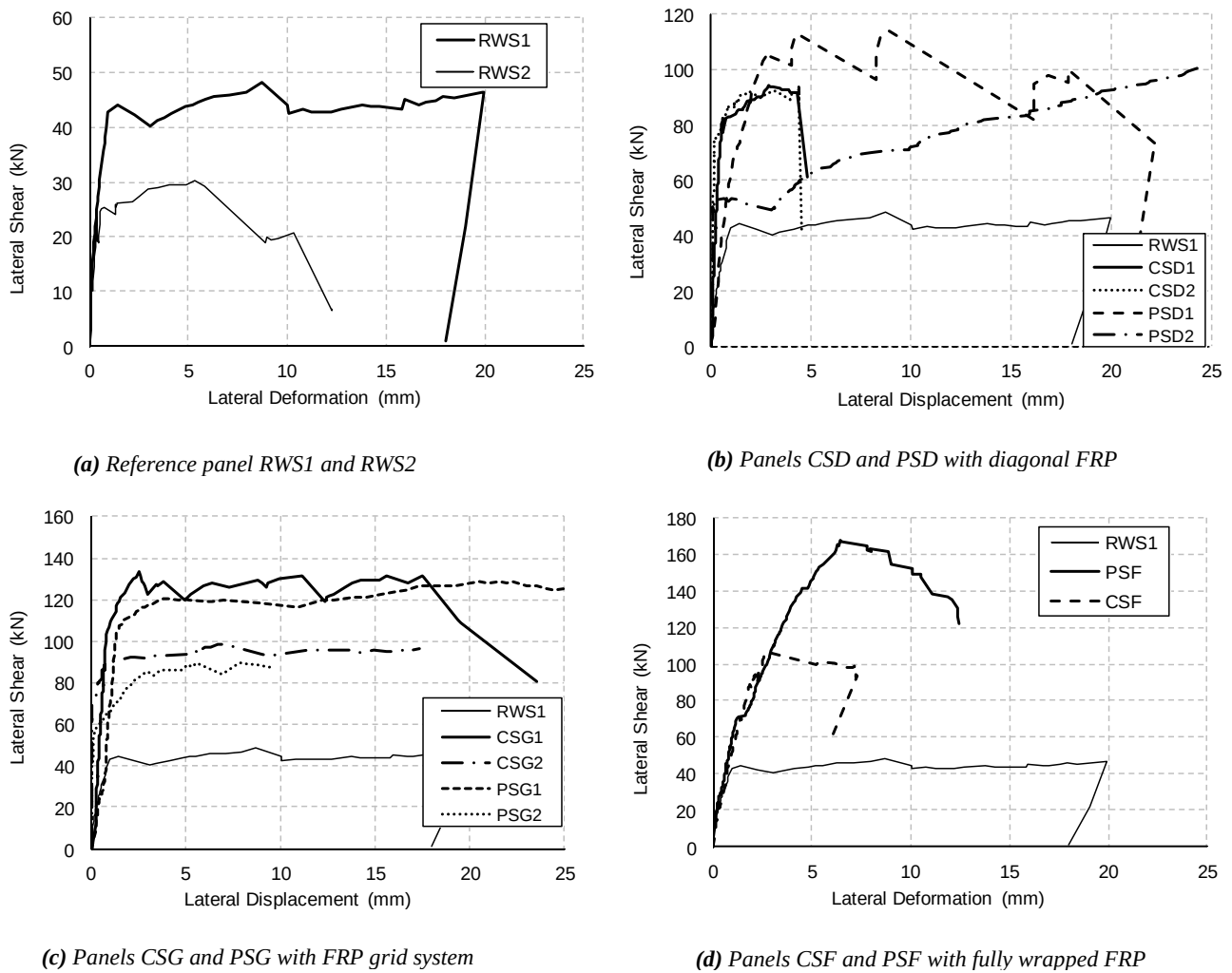
Fig. 12. Load-deformation responses of unreinforced and retrofitted masonry shear walls
