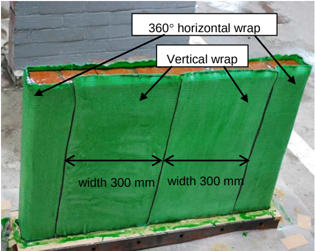
Fig. 8. FRP installation in fully wrapped wall
