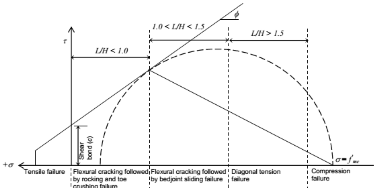
Fig. 2. Generalized behavior of URM under combined shear and normal stress
