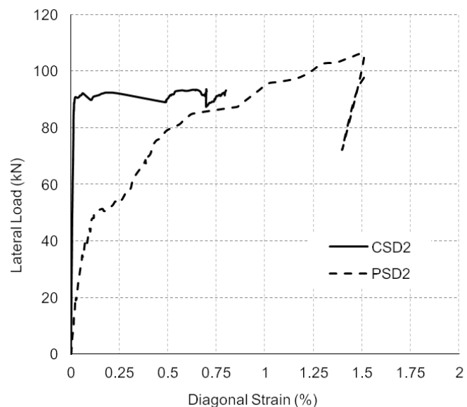
Fig. 14. Load–strain responses in diagonal FRP strips of retrofitted panels at point 2 on Fig. 9(a)
