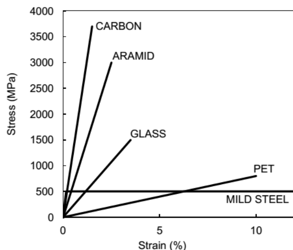
Fig. 3. Tensile strength of different FRPs
