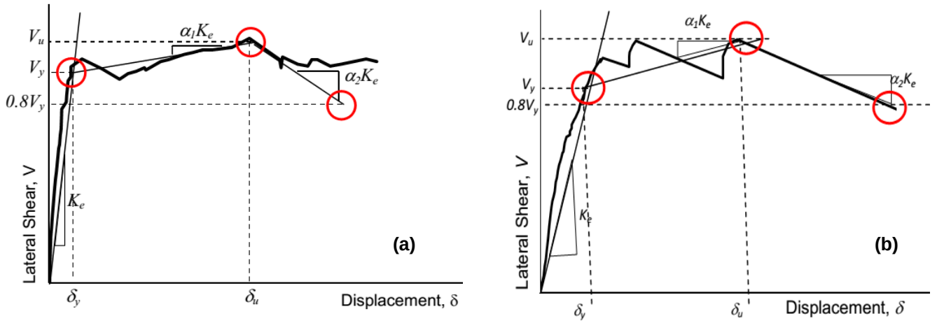
Fig. 17. Idealized force-displacement curve for (a) RWS1 and (b) CSD1 panels
