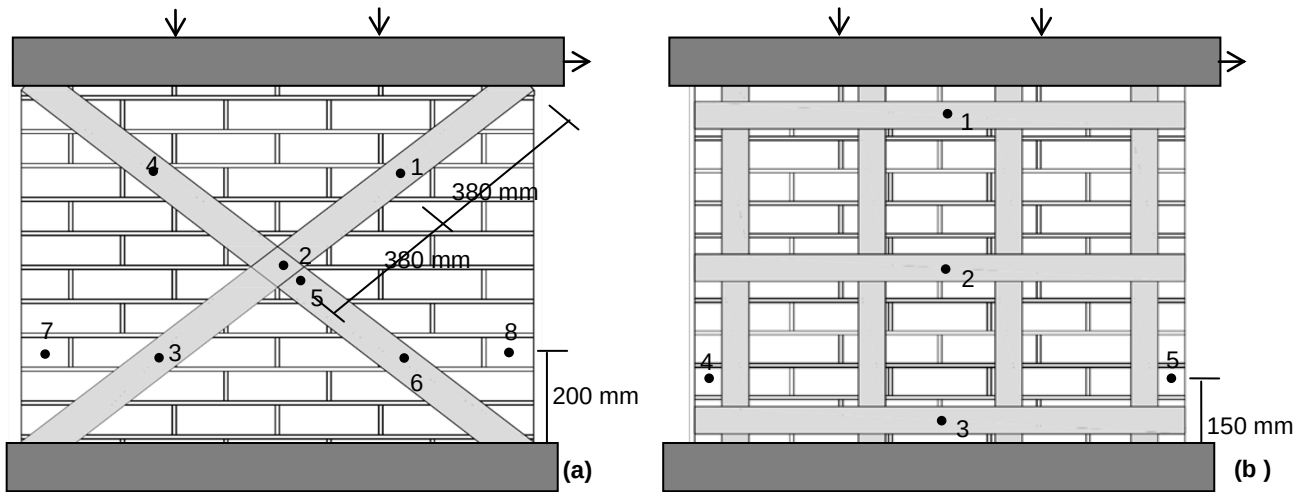
Fig. 9. Strain gauges layout (a) cross digonal layout (b) grid layout
