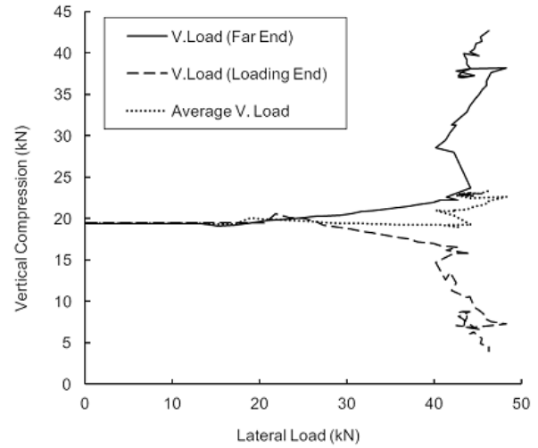
Fig. 13. Variation of vertical load with progressive shear
