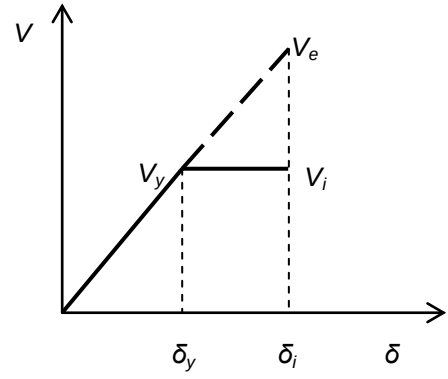
Fig. 16. Equal displacement rule for linear elastic analysis
