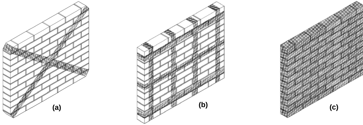
Fig. 5. FRP reinforcement layout, (a) FRP cross diagonal bracings (CSD, PSD); (b) FRP strips in grid system (CSG, PSG); (c) Fully wrapped by FRP (CSF, PSF)
