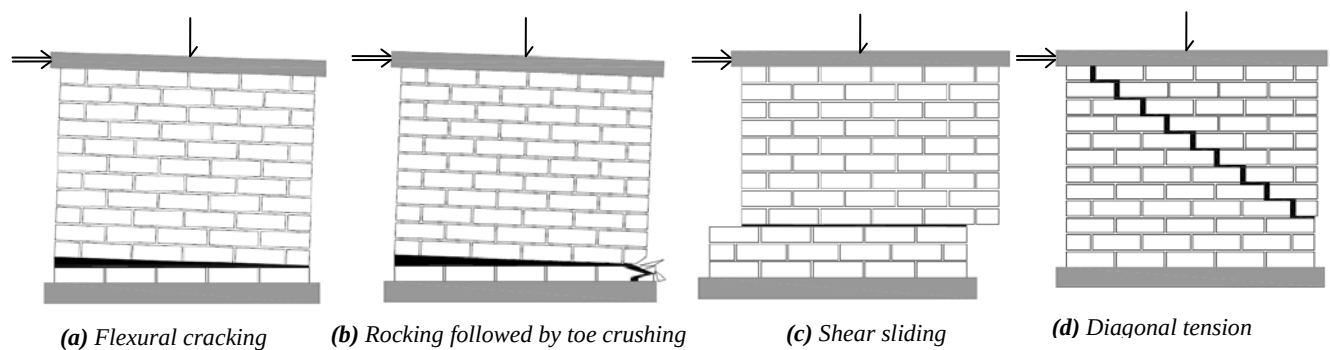
Fig. 1. Different Failure modes of URM
