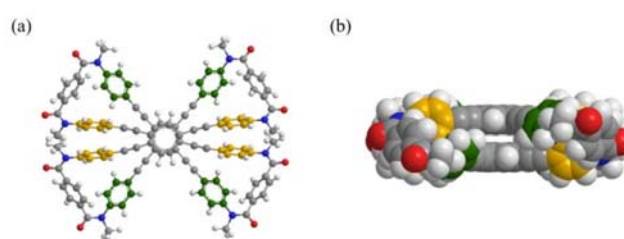
Fig. 3 The most energy-minimized structure for 2' [X = Y = Me]: (a) top view (ball and stick representation) and (b) side view (space-filling representation), obtained by a conformational search using MacroModel software (v9.9 OPLS_2005, Monte Carlo Multiple Minimum method, non-solvated, 50 000 steps). Only one enantiomeric form with ( M )-helicity is depicted.
