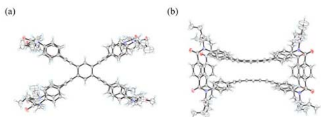
Fig. 2 X-ray structure of 2 [X = Y = n Bu]: (a) top view and (b) side view. Solvents are omitted for clarity.
