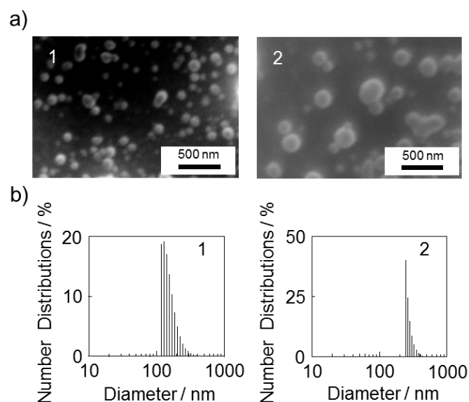
Fig. 3 a) SEM images of 1 : [\text{Eu}(\text{hfa})_3(\text{dpbb})_x(\text{SDPO})_y]_n and 2 : [\text{Eu}(\text{hfa})_3(\text{dpbb})_x(\text{SDPO})_y]_n\text{-PS} . b) Number distributions of 1 : [\text{Eu}(\text{hfa})_3(\text{dpbb})_x(\text{SDPO})_y]_n and 2 : [\text{Eu}(\text{hfa})_3(\text{dpbb})_x(\text{SDPO})_y]_n\text{-PS} using DLS measurements.
