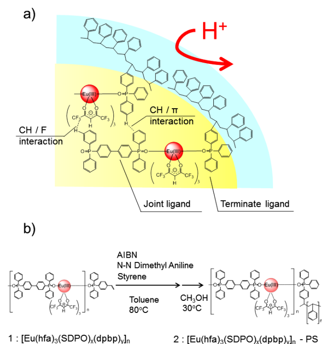
Fig. 1 Preparation scheme of acid protected lanthanide coordination nanoparticles covered with polystyrene.
