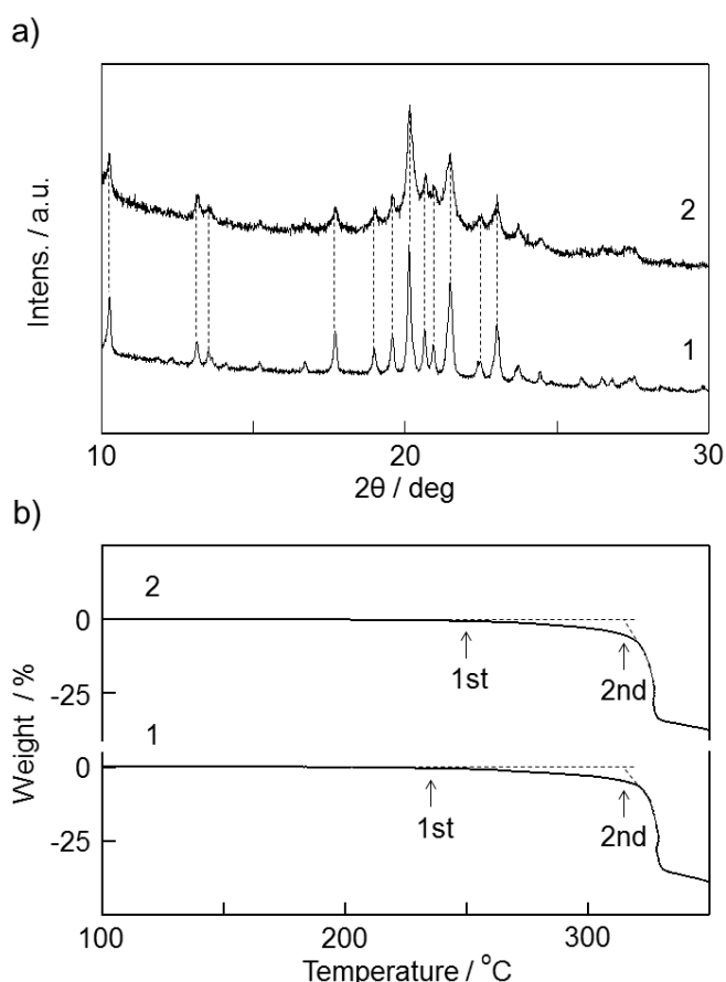
Fig. 2 a) XRD patterns of 1 : [\text{Eu}(\text{hfa})_3(\text{dpbb})_x(\text{SDPO})_y]_n and 2 : [\text{Eu}(\text{hfa})_3(\text{dpbb})_x(\text{SDPO})_y]_n\text{-PS} . b) TGA curves of 1 : [\text{Eu}(\text{hfa})_3(\text{dpbb})_x(\text{SDPO})_y]_n and 2 : [\text{Eu}(\text{hfa})_3(\text{dpbb})_x(\text{SDPO})_y]_n\text{-PS} in argon atmosphere at a heating rate of 2^\circ\text{C min}^{-1} .
