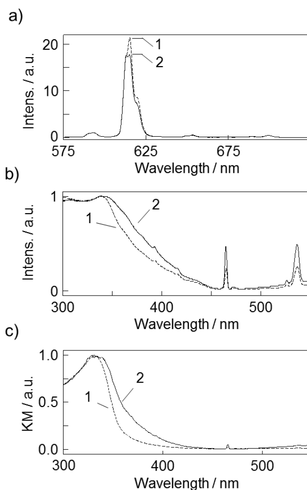
Fig. 4 a) Emission spectra of 1 : [\text{Eu}(\text{hfa})_3(\text{dpbp})_x(\text{SDPO})_y]_n and 2 : [\text{Eu}(\text{hfa})_3(\text{dpbp})_x(\text{SDPO})_y]_n\text{-PS} in solid state at room temperature. Excited at 370 nm. b) Excitation spectra of 1 : [\text{Eu}(\text{hfa})_3(\text{dpbp})_x(\text{SDPO})_y]_n and 2 : [\text{Eu}(\text{hfa})_3(\text{dpbp})_x(\text{SDPO})_y]_n\text{-PS} in solid state at room temperature. Monitored at 613 nm. c) Diffuse reflection spectra of 1 : [\text{Eu}(\text{hfa})_3(\text{dpbp})_x(\text{SDPO})_y]_n and 2 : [\text{Eu}(\text{hfa})_3(\text{dpbp})_x(\text{SDPO})_y]_n\text{-PS} in solid state at room temperature.
