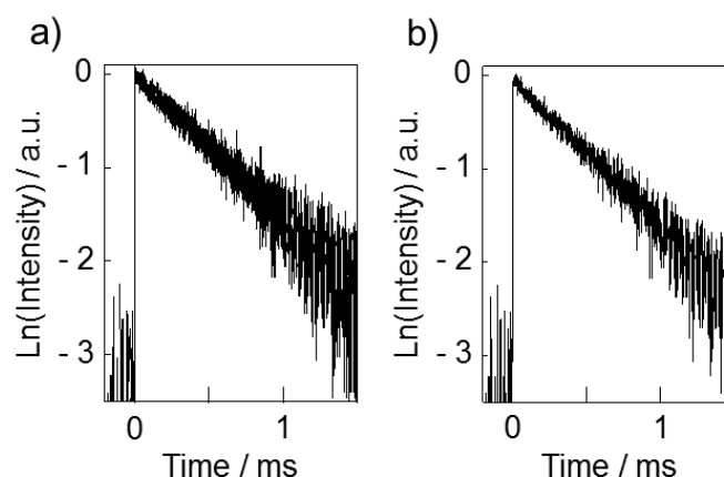
Fig. 5 Emission decays of a): [\text{Eu}(\text{hfa})_3(\text{dpbbp})_x(\text{SDPO})_y]_n and b): [\text{Eu}(\text{hfa})_3(\text{dpbbp})_x(\text{SDPO})_y]_n\text{-PS} in solid state at room temperature excited at 355 nm (third harmonic of a Q-switched Nd:YAG laser: fwhm = 5 ns, \lambda = 1064 nm).
