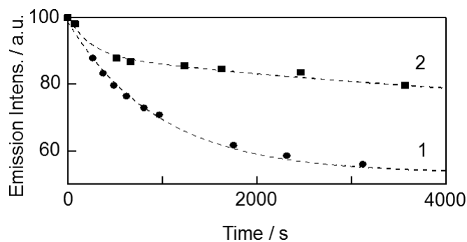
Fig. 6 Time dependences of the emission intensities of 1: [\text{Eu}(\text{hfa})_3(\text{dpbbp})_x(\text{SDPO})_y]_n (circles) and 2: [\text{Eu}(\text{hfa})_3(\text{dpbbp})_x(\text{SDPO})_y]_n\text{-PS} (squares) under Acidic condition (pH = 0.92).
