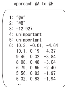
Figure 9: move-close-to
