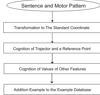
Figure 4: Movement Cognition
