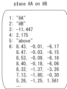
Figure 8: place-on
