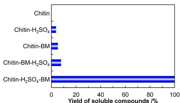
Figure 1. Mechanocatalytic depolymerization of chitin. Dissolution conditions: chitin weight 406 mg; distilled water 40 mL; 298 K.
