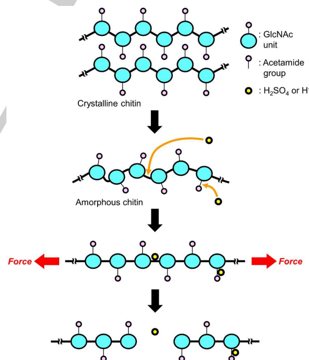
Scheme 2. Proposed schematic of mechanochemical depolymerization. The mechanical force first amorphizes chitin, which increases the accessibility of acid to the substrate. The main chain is subjected to strong mechanical force, which leads to selective dissociation of the connecting points of the chain (glycosidic bonds), while the side chains (acetamide groups) do not dissociate.
