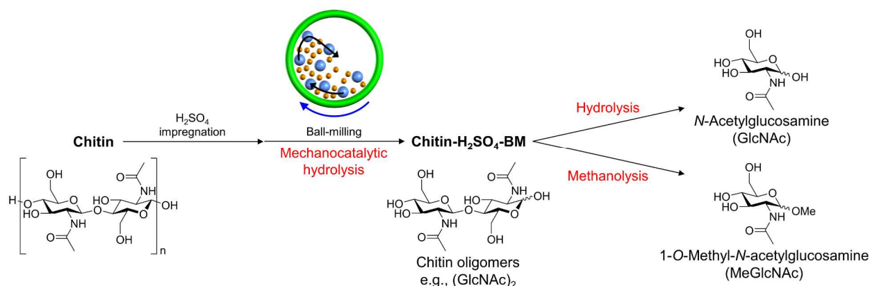
Scheme 1. Two-step depolymerization of chitin to N -acetylated monomers, catalyzed by \text{H}_2\text{SO}_4 . The first step is mechanocatalytic depolymerization of chitin to water-soluble oligomers, and the second is solvolysis of the oligomers to N -acetylated monomers.
