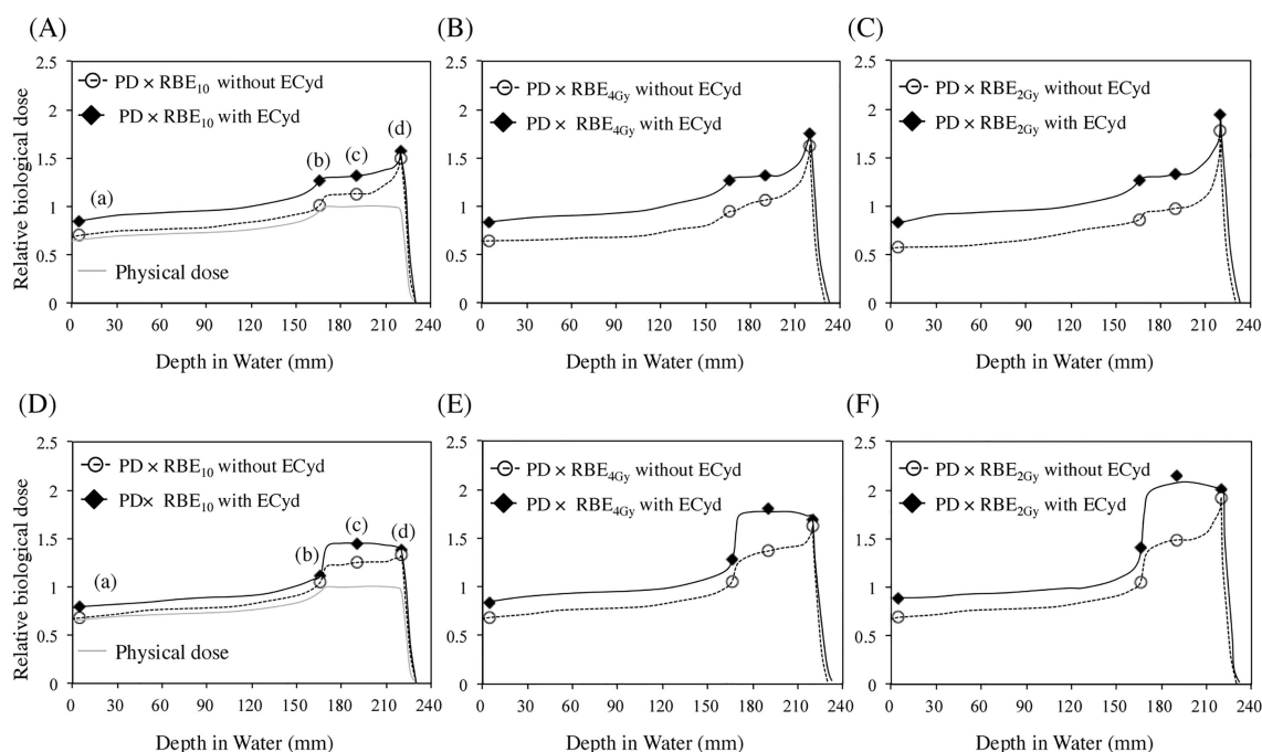
Fig 3. Relative dose-depth distributions. Dose-depth distributions in A549 cells (A)–(C) and V79 cells (D)–(F). Relative physical dose (PD) (gray solid line), PD × relative biological equivalent (RBE) in the absence of ECyd (white circle and dotted-line), PD × RBE in the presence of ECyd (black diamond shape and black solid line) at each depth ((a) through (d), as shown in Fig 1B) of the proton beam. The physical dose was normalized at the center of the spread-out Bragg peak. The values shown in S1 Table were used for RBE values [RBE 10 for (A) and (D), RBE 4Gy for (B) and (E), RBE 2Gy for (C) and (F)].
