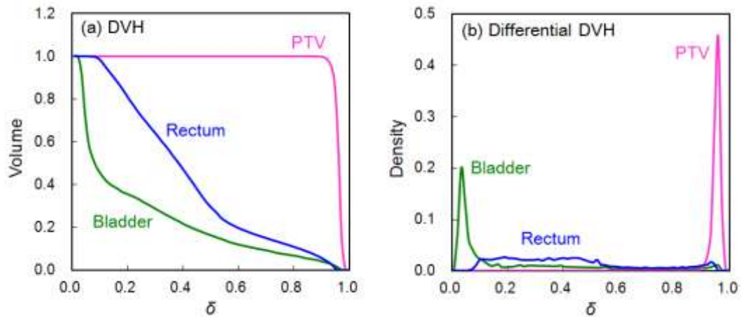
225 FIG. 1. Example of the dose volume histogram for treatment of prostate cancer: (a) dose volume histograms (DVHs) for bladder, rectum and planning target volume (PTV), (b) differential dose volume histograms for bladder, rectum and PTV.
