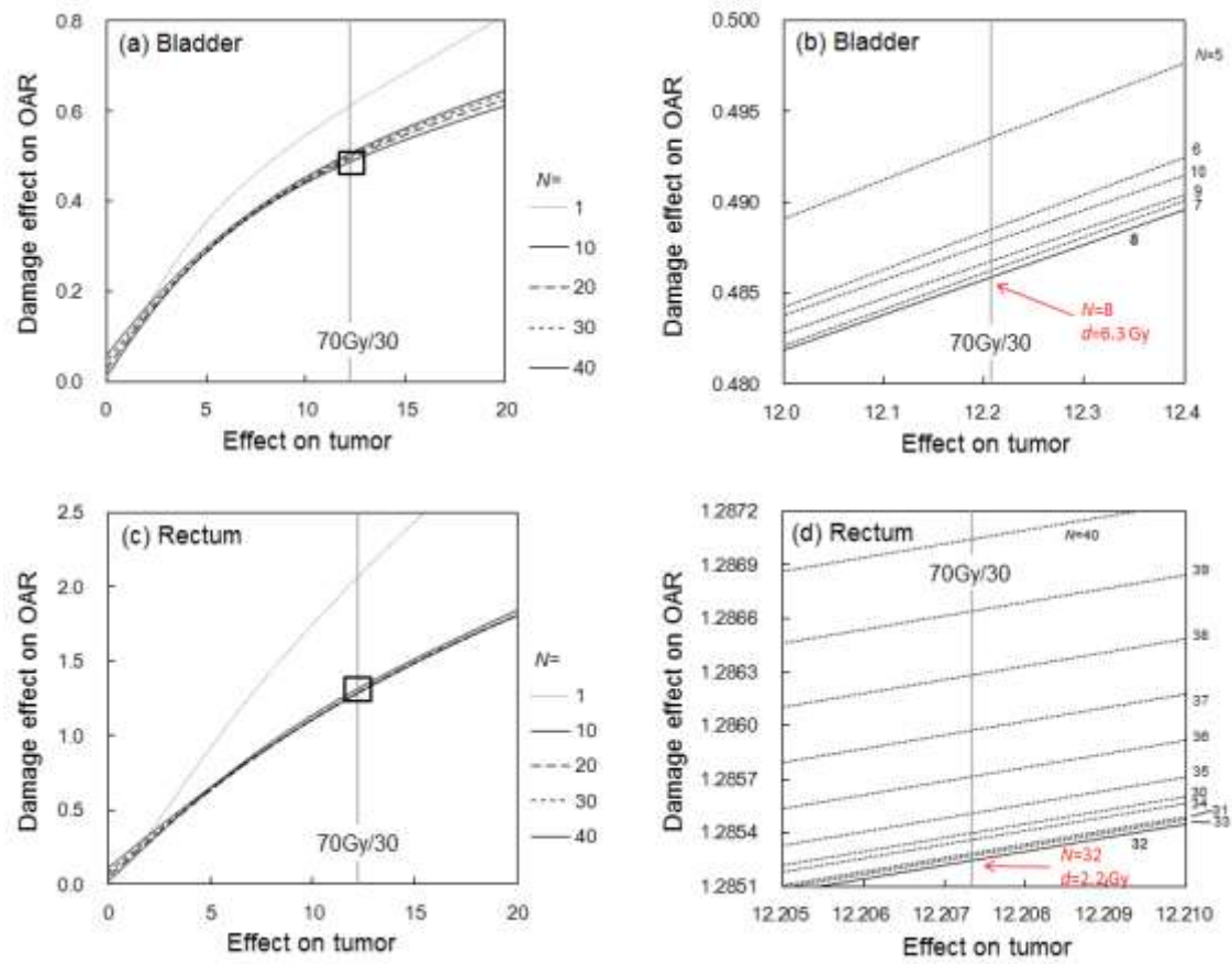
FIG. 4. TO plots for bladder and rectum calculated with USC-repopulation model. (a) TO plot for bladder, (b) Enlarged view of TO plot for bladder (□ area in (a)), (c) TO plot for rectum, (d) Enlarged view of TO plot for rectum (□ area in (c)). ( N : Number of fractions)
