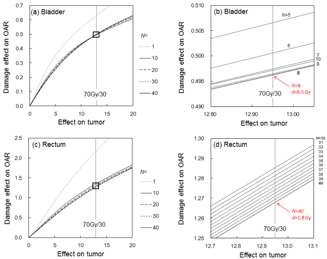
FIG. 3. TO plots for bladder and rectum calculated with USC model. (a) TO plot for bladder, (b) Enlarged view of TO plot for bladder ( \square area in (a)), (c) TO plot for rectum, (d) Enlarged view of TO plot for rectum ( \square area in (c)). ( N : Number of fractions)
