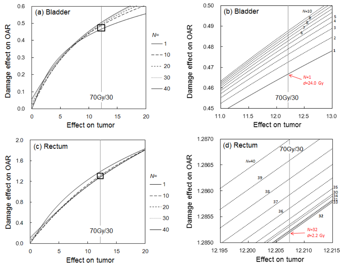
FIG. 2. TO plots for bladder and rectum calculated with LQ-repopulation model.
