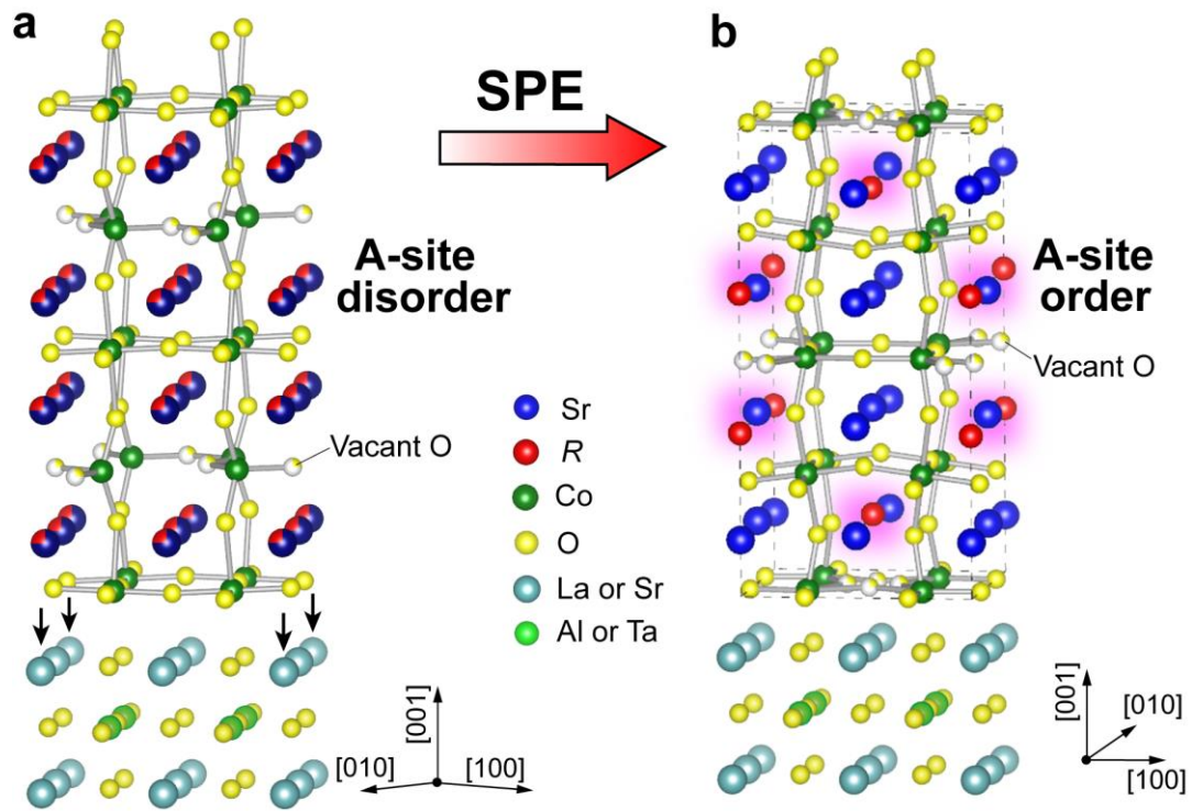
Figure 1. Schematic illustration of the strategy to produce epitaxial SRCO films with well-aligned A-site-ordered structure on (La,Sr)(Al,Ta)O 3 substrates; this was undertaken by solid-phase epitaxy (SPE) with two-step film-synthesis process combining low- T epitaxial growth and a subsequent high- T annealing. Here, the ideal crystal structure of A-site-ordered Sr 3 RCO 4 O 10.5 is shown. (a) the A-site-disordered perovskite framework of SRCO with oxygen-vacancy ordered structure (brownmillerite(BM)-type structure) is epitaxially grown on the substrates. (b) SRCO film with an A-site-ordered structure, obtained by high- T annealing of the as grown film with BM-type structure in air. The dashed line indicates the unit cell of A-site-ordered SRCO. In this study, Er was selected as element R . Crystalline orientations for as-grown [24] and SPE grown SECO films [7] are shown at the bottom right of each figure.
