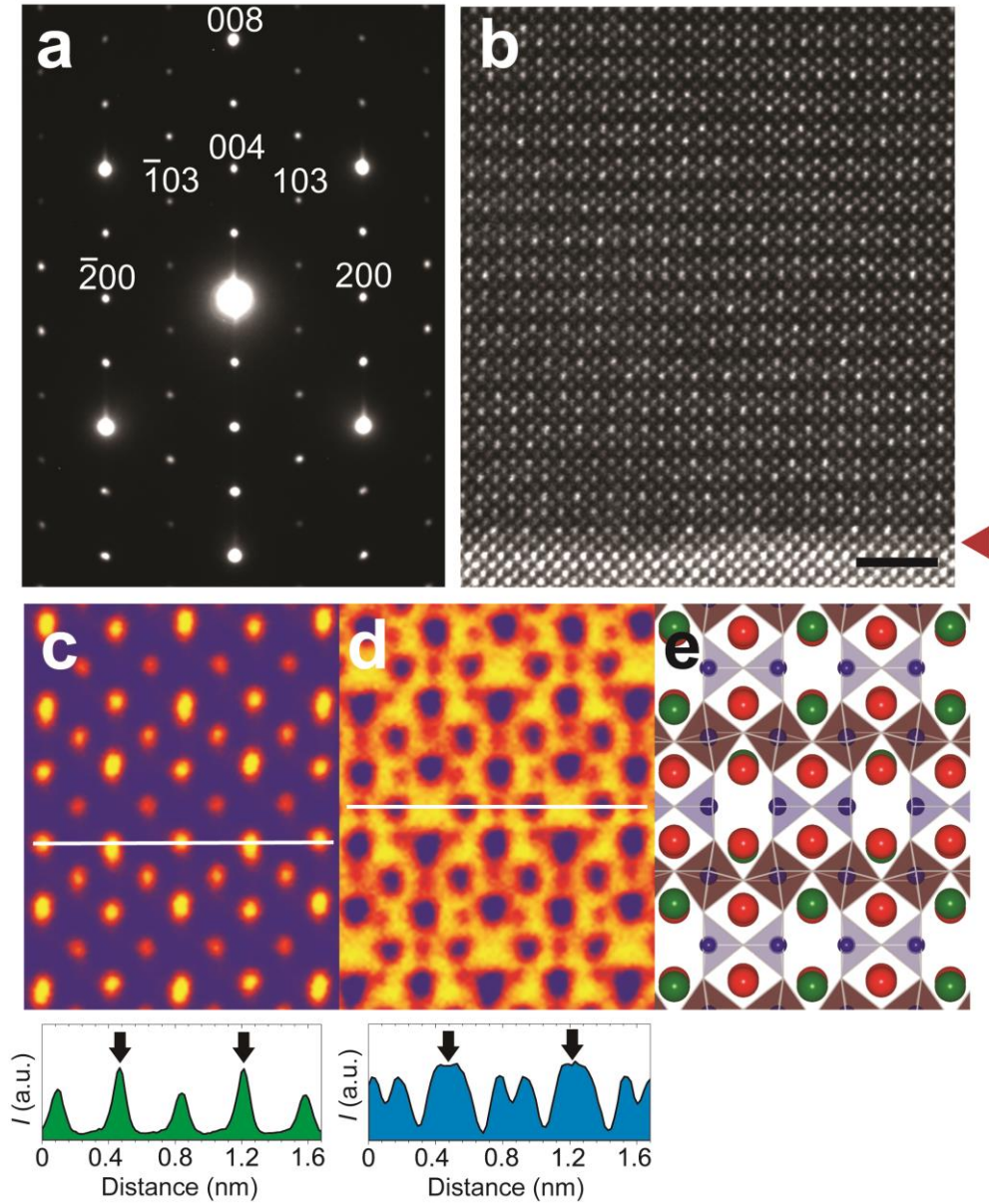
Figure 3. High-resolution STEM analyses of the SPE-grown SECO epitaxial films on LSAT substrates. (a) Selected-area electron diffraction pattern of the film with the main diffraction spots from SECO assigned. (b) Cross-sectional HAADF-STEM image (scale bar = 2 nm) — the red triangle denotes the position of the heterointerface. (c) Magnified HAADF-STEM and (d) ABF-STEM images, which are obtained by averaging 20 original HAADF and ABF images. These images are representative of the ordered structure observed in wide area of the SECO film. The bottom panels of (c) and (d) show HAADF and ABF intensity profiles, respectively, collected along the white lines in each image. The black arrows indicate the positions of Sr/Er columns and oxygen-vacancy columns in each panel. (e) A schematic illustration of the atomic structure of the ordered SECO.
