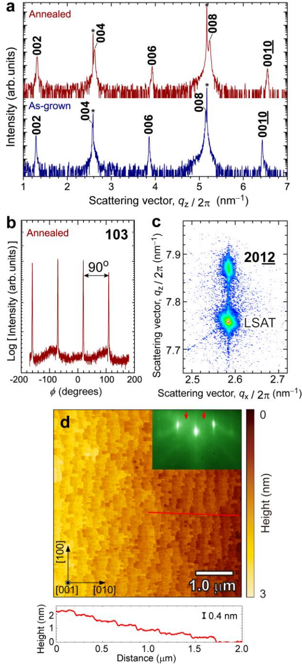
Figure 2. Structural characterization for SECO films as-grown ( T_g = 820 °C, P_{O_2} = 10 Pa) and SPE-grown ( T_a = 1050 °C) at well-optimized conditions. (a) Out-of-plane XRD patterns of as-grown (blue) and SPE-grown (red) films. Diffraction indices are noted above the corresponding diffraction peaks. LSAT substrate peaks are indicated by asterisks (*). The double lattice spacing along the c -axis ( l = 2, 6, 10 ) originates from the oxygen-vacancy ordering. (b) In-plane \phi -scans for the asymmetric reflection of 103 diffraction peaks of the SPE-grown SECO films. The four diffraction peaks with 90° rotational intervals observed in the SPE-grown film are attributed to A-site ordering. (c) Reciprocal space mapping around 2012 A-site-ordered SECO for the SPE-grown film. (d) Topographic AFM image of the SPE-grown SECO film. Below: Height profile derived from the red line on the image. Inset: RHEED pattern from this film, confirming the atomically flat surface of the SPE-grown SECO film. The arrows indicate the position of weak diffraction spots originating from the superstructure (A-site-ordered structure) of film surface and/or surface reconstruction.
