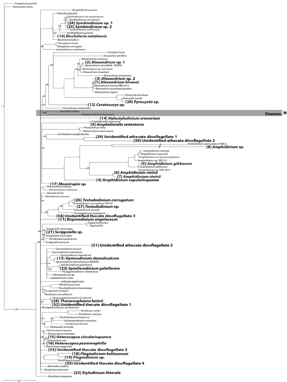
Fig. S3 The Bayesian molecular phylogeny inferred from SSU rDNA of Dinophyta including peridinin-type dinoflagellates and dinotoms Numbers on the major nodes represent posterior probability. Only PP>0.5 is shown. Analyzed strains and numbers are shown by bold type. Gray boxes with asterisk indicate dinotoms.
