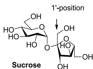
Figure 6.1 Sucrose and the 1'-position
