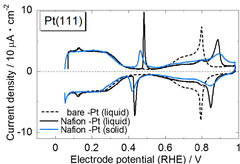
Fig. 5.2.2 The CVs for the Nafion-coated Pt (111) surfaces in the aqueous (liquid) electrolyte of 0.1 M \text{HClO}_4 (black solid line) and in the solid-state cell (blue solid line). The CV for a bare Pt (111) is also shown for comparison (black dashed line).
