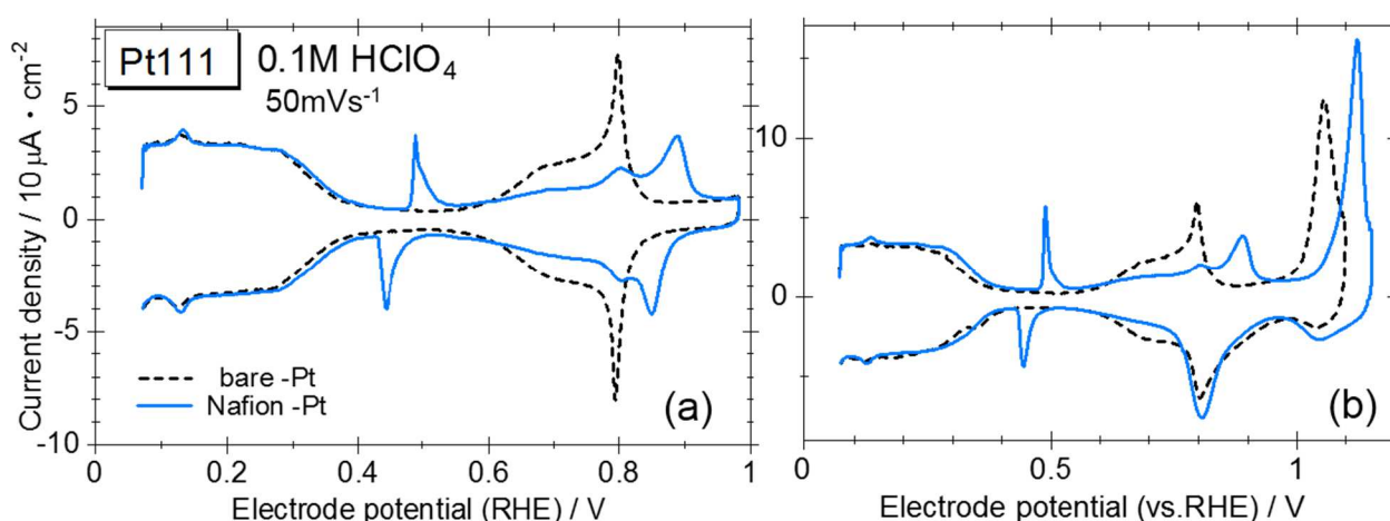
Fig. 5.1.2 CVs for Pt (111) surfaces with and without the Nafion coating. Upper limit of the potential scan: (a) 0.98 V, (b) 1.15 V. Blue solid line: with Nafion coating, black dashed line: without Nafion coating (bare-Pt).
