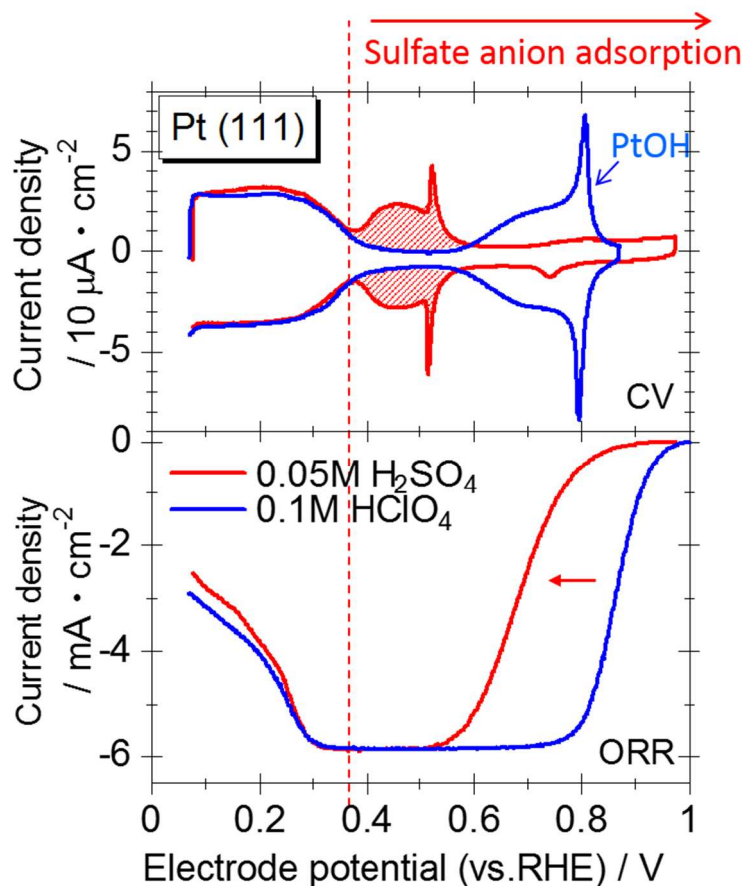
Fig. 5.1 The effect of sulfate anion adsorption on the CV and ORR curve on Pt (111) surface. The shaded butterfly peaks correspond to the oxidative adsorption and reductive desorption of sulfate. ORR activity is significantly suppressed by the anion adsorption.
