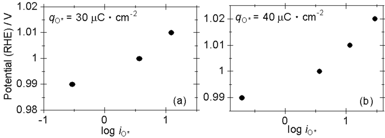
Fig. 3.1.8 Tafel plots for the oxide formation at (a) 30 and (b) 40 \mu\text{C} \cdot \text{cm}^{-2} .
