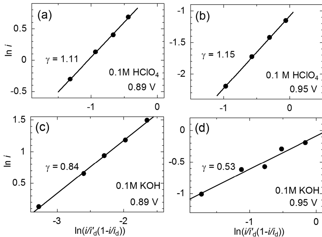
Fig. 3.2.4 Typical plots of \ln i vs. \ln\{i_d(1-i/i_d)/i_d\} . (a) The plots at 0.89 V in 0.1 M HClO 4 , (b) those at 0.95 V in 0.1 M HClO 4 , (c) those at 0.89 V in 0.1 M KOH and (d) those at 0.95 V in 0.1 M KOH.
