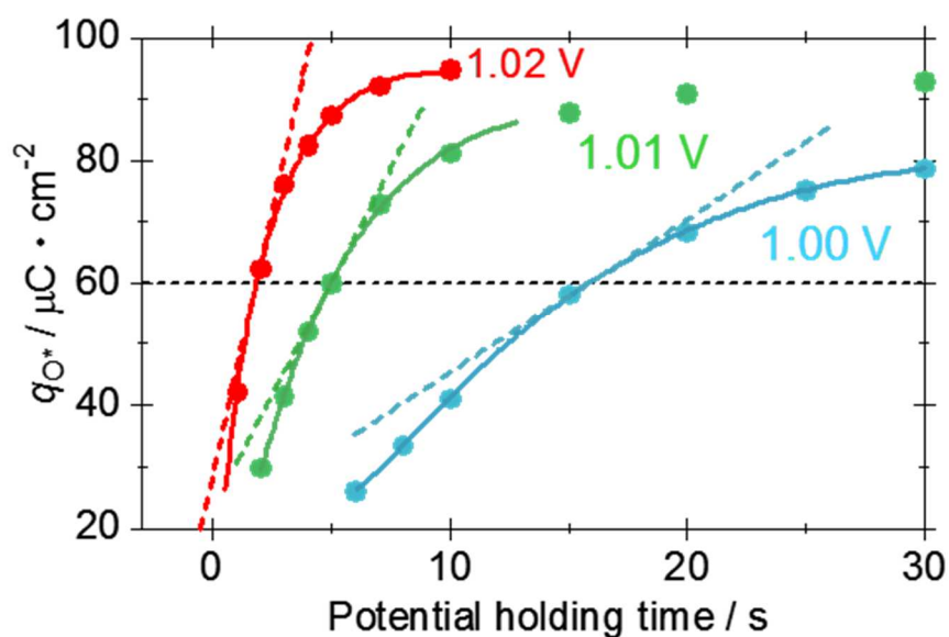
Fig. 3.1.6 The estimation procedure for the oxide formation current densities at the oxide amount of 60 \mu C \cdot cm^{-2} . Solid lines: the locally fitted curves. Dashed lines: the tangents at 60 \mu C \cdot cm^{-2} whose slopes are equal to the oxide formation current densities: 2.5, 7.4 and 17 \mu A \cdot cm^{-2} at the electrode potentials of 1.00, 1.01 and 1.02 V.
