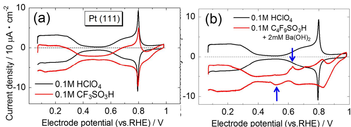
Fig. 5.4.9 The CVs of a bare Pt (111) in (a) 0.1 M TFMSA and (b) 0.1 M NFBSA with the additive of \text{Ba}(\text{OH})_2 (red solid curves). The CV in 0.1 M \text{HClO}_4 is also shown for comparison (black solid curves).
