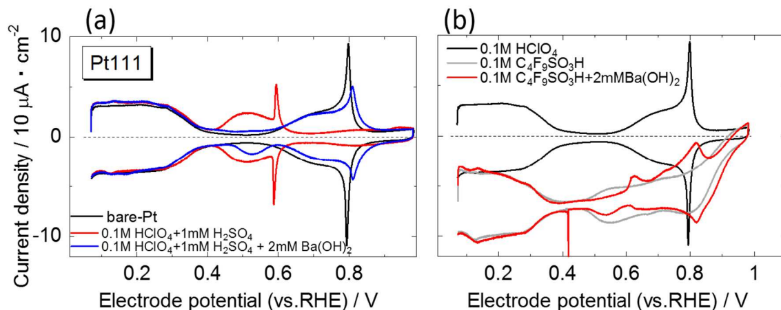
Fig. 5.4.10 The effect of the addition of Ba cation for precipitating the impurity of sulfate anion. (a) Sulfate anion with the concentration of 1 mM is significantly adsorbed on Pt (111) as shown by the appearance of sulfate-derived butterfly peaks between 0.4 – 0.6 V and the disappearance of hydroxide-derived ones between 0.6 – 0.85 V in the red curve. With the addition of 2 mM of \text{Ba}(\text{OH})_2 , the sulfate-derived butterfly peaks attenuate and the hydroxide-derived ones re-appear. The suppression of the adsorption of sulfate anions is surely due to precipitation of sulfate anion with Ba cations. (b) The CV of Pt (111) in 0.1 M NFBSA without the additive of \text{Ba}(\text{OH})_2 (gray solid curve) shows broad peaks between 0.5 – 0.8 V and the disappearance of the hydroxide-derived butterfly peaks. The broad peak is attenuated by the addition of \text{Ba}(\text{OH})_2 (red solid curve) and therefore ascribed to the impurity of sulfate anion.
