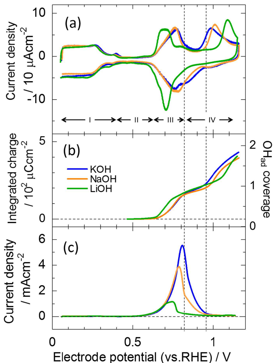
Fig.4.1.1 The effects of alkali metal cations on CVs and MOR currents in alkaline solution on Pt (111). (a) The effects on the shape of CV, including H upd (region I), the double layer (region II), reversible adsorption of OH (region III) and irreversible oxide formation (region IV). (b) The effects on surface coverage of OH ad . (c) The effects on polarization curves for MOR. The vertical dashed lines at 0.82 and 0.95 V emphasize that at a similar OH ad coverage, the activities of MOR are controlled only by the nature of the cations.
