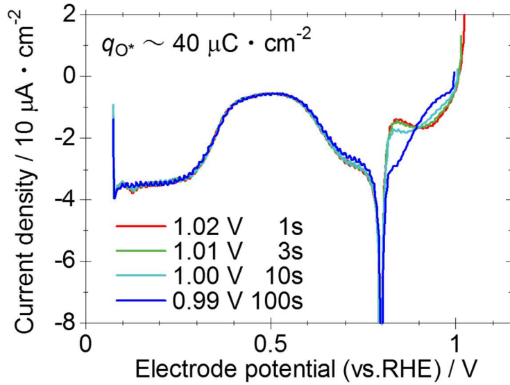
Fig. 3.1.9 The cathodic linear sweep voltammograms where q_{\text{O}^*} 's are close to 40 \mu\text{C} \cdot \text{cm}^{-2} . The hold potentials are 0.99 V (blue), 1.00 V (light blue), 1.01 V (green) and 1.02 V (red).
