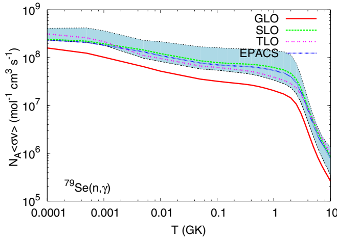
FIG. 10. ^{79}\text{Se}(n, \gamma) reaction rates as a function of temperature, calculated by using the code TALYS with various models for the input strength function. The uncertainty of the EPACS shown as a blue band results from the use of various nuclear level density models.
