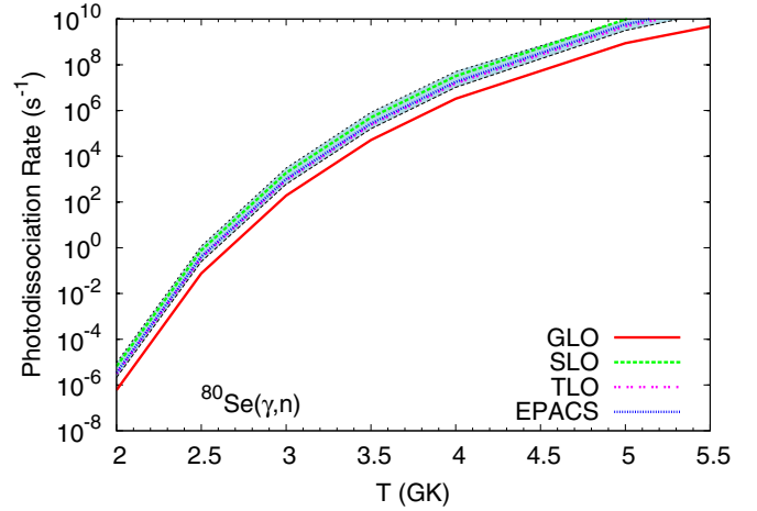
FIG. 11. ^{80}\text{Se}(\gamma, n) reaction rates as a function of temperature, calculated by using the code TALYS with various models for the input strength function. The uncertainty of the EPACS shown as a blue band results from the use of various nuclear level density models.
