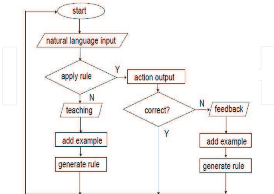
Fig. 7. System flowchart
