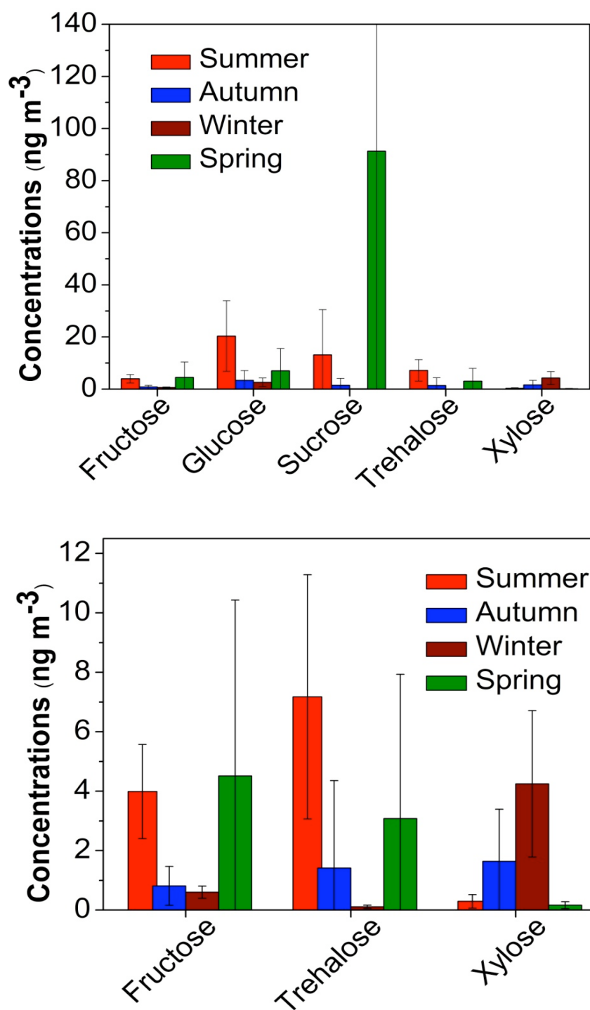
Fig. 7. Seasonal variations of primary sugars in Alaska aerosols
