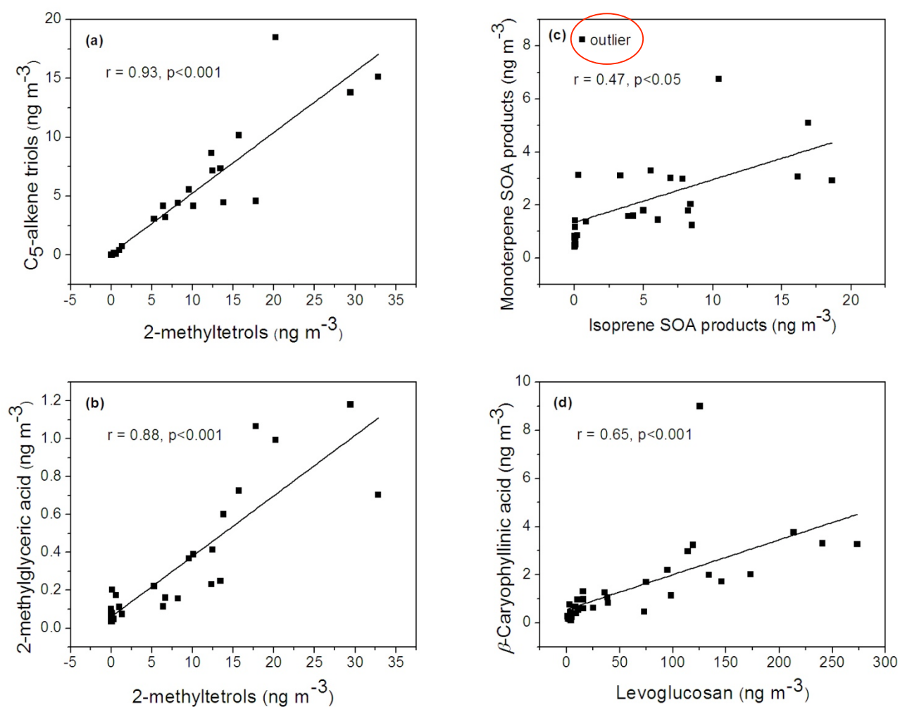
Fig. 4. Relations between (a) C 5 -alkene triols and 2-methyltetrols, (b) 2-methylglyceric acid and 2-methyltetrols, (c) monoterpene SOA products and isoprene SOA products, and (d) \beta -caryophyllinic acid and levoglucosan.
