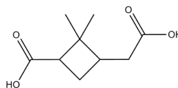
Pinic acid
