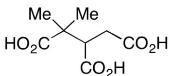
3-Methyl-1,2,3-butanetricarboxylic acid (MBTCA)
