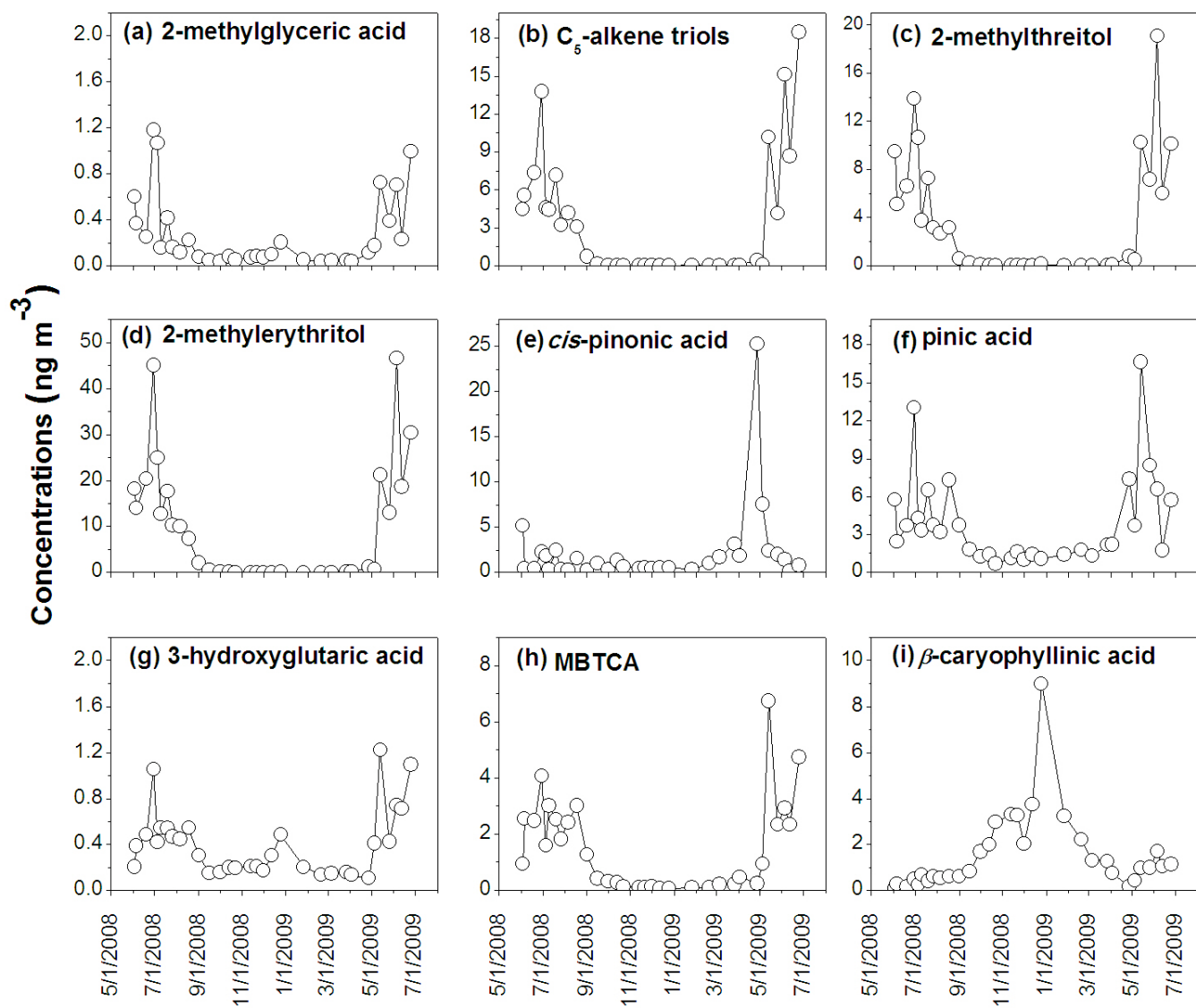
Fig. 3. Temporal variations of biogenic SOA tracers measured in the Alaskan aerosols.
