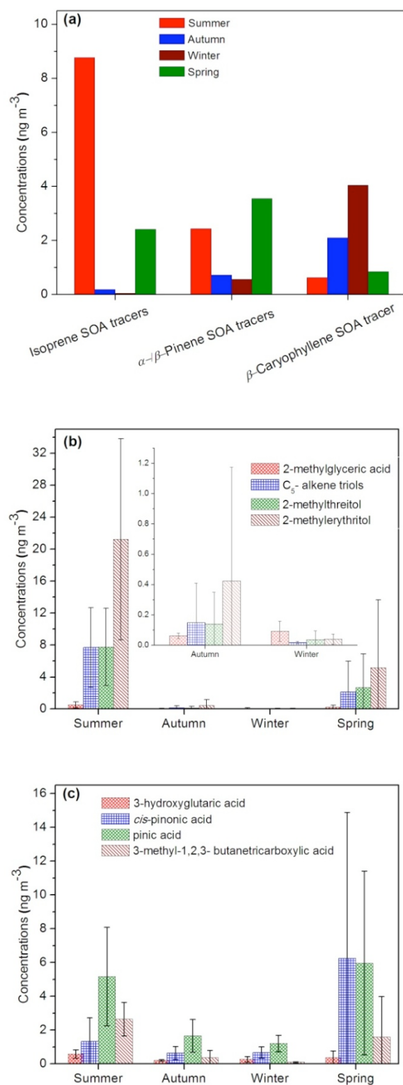
Fig. 5. Seasonal variations of (a) isoprene, \alpha - \beta -pinene and \beta -caryophyllene SOA tracers, (b) isoprene SOA tracers, and (c) \alpha - \beta -pinene SOA tracers.
