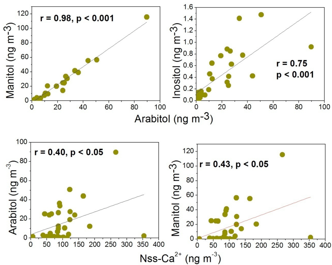
Fig. 6. Correlations among arabinitol, manitol, inositol, and nss-Ca 2+ in Alaska aerosols.
