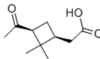
Pinonic acid
