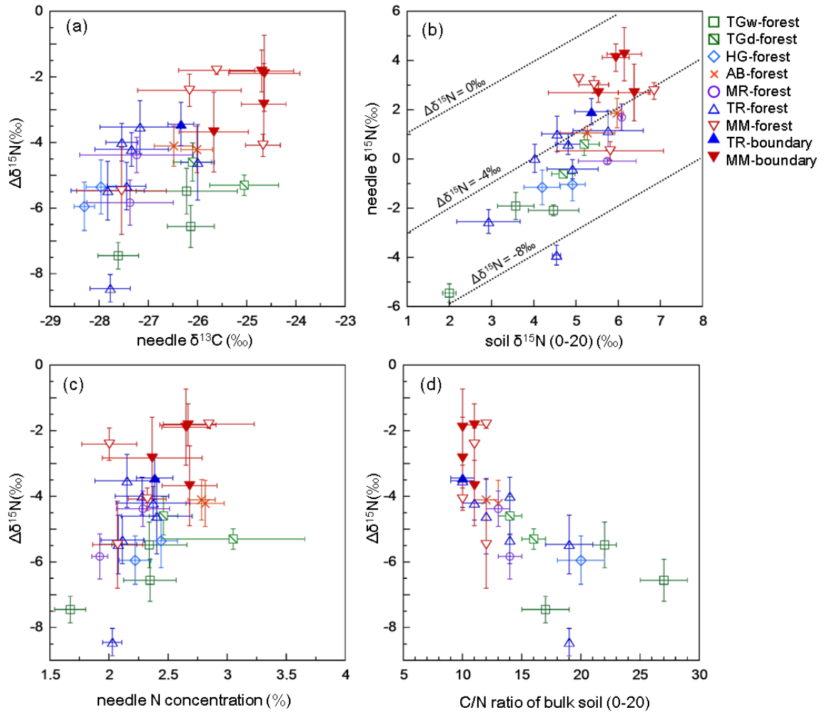
Figure 3.7. Correlations between larch needle \delta^{13}\text{C} and \Delta\delta^{15}\text{N} ( r_s = 0.648 ) (a), needle and soil \delta^{15}\text{N} ( r_s = 0.795 ) (b), needle N concentration and \Delta\delta^{15}\text{N} ( r_s = 0.499 ) (c), and C/N ratio of bulk soil and \Delta\delta^{15}\text{N} ( r_s = -0.793 ) (d) at all sites in all areas. Dotted lines in (b) indicate \Delta\delta^{15}\text{N} values at 0‰, -4‰ and -8‰. Correlation coefficients are significant at p < 0.05 . Bars represent standard deviation of the mean.
