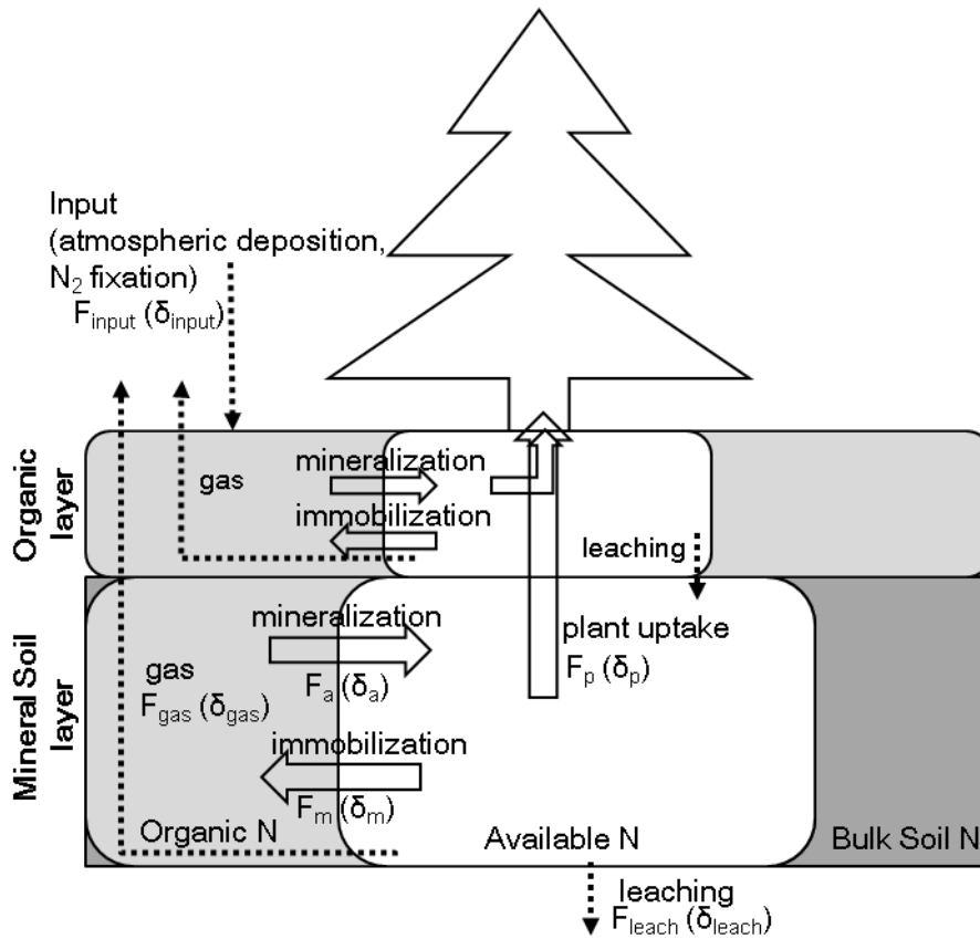
Figure 2.10. Schematic representation of the N cycle in the plant-soil system. Arrows with its flux and \delta^{15}N in parentheses are the processes that included in the mass balance. White arrows are the processes within the system, whereas black dotted arrows are the processes of N input and loss. Under the rapid decomposition of organic matter in grassland boundary, most of the available N produced in the soil ( F_a ) is transported to larch ( F_p ) without significant N isotope fractionation ( \delta_a = \delta_p = \delta_m ), leading to small \Delta\delta^{15}N . Under the significant accumulation of organic layer in forest, the ^{15}N -depleted part of available N is transported to larch ( F_p ), whereas the ^{15}N -enriched part remains in the soil immobilized by microorganisms ( F_m ) ( \delta_p < \delta_m ), leading to large \Delta\delta^{15}N .
