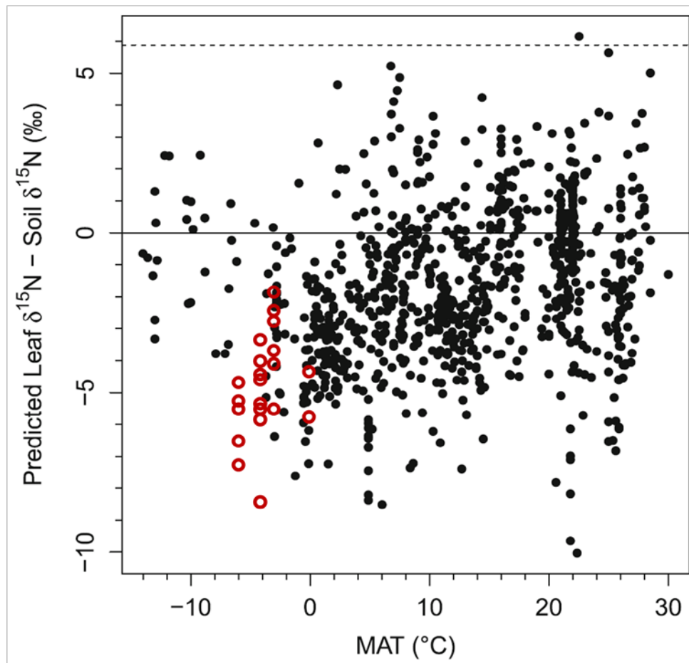
Figure 4.3. Relationship between mean annual temperature (MAT) and the difference between \delta^{15}\text{N} of leaves and soil in Craine et al. (2015). In this figure, the data obtained in this study were plotted as red circle. MAT was -6^{\circ}\text{C} in TG area, -4^{\circ}\text{C} in HG, AB, TR area, -3^{\circ}\text{C} in MM area, and 0^{\circ}\text{C} in MR area.
