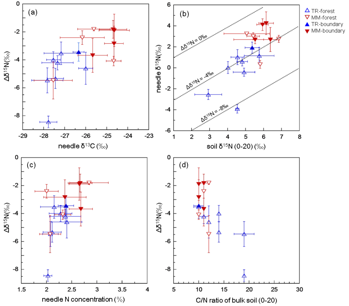
Figure 3.6. Correlations between larch needle \delta^{13}\text{C} and \Delta\delta^{15}\text{N} ( r_s = 0.753 ) (a), needle and soil \delta^{15}\text{N} ( r_s = 0.718 ) (b), needle N concentration and \Delta\delta^{15}\text{N} ( r_s = 0.591 ) (c), and C/N ratio of bulk soil and \Delta\delta^{15}\text{N} ( r_s = -0.541 ) (d) at all sites in TR area and MM area.
