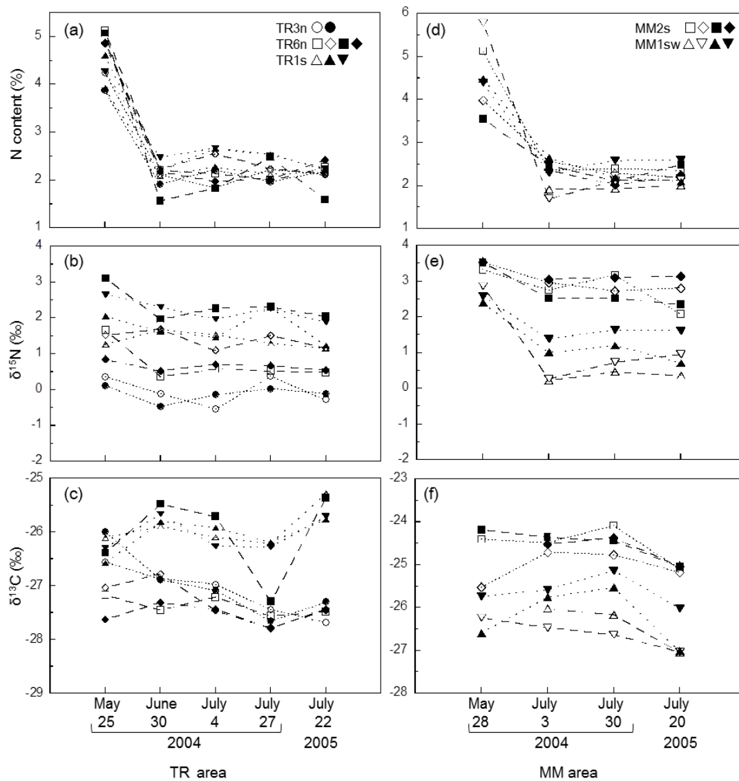
Figure 3.1. Temporal variations in larch needle N concentration (a), \delta^{15}\text{N} (b), and \delta^{13}\text{C} (c) in TR area, and the same as (d), (e), and (f) in MM area. Data from two trees at TR3n, four trees at TR6n, and three trees at TR1s in TR area, as well as four trees at MM1sw and four trees at MM2s in MM area were shown. Each tree was expressed by a different shape (circle, rectangle, or triangle) and colour (black or white). Trees within the same site share the same shape.
