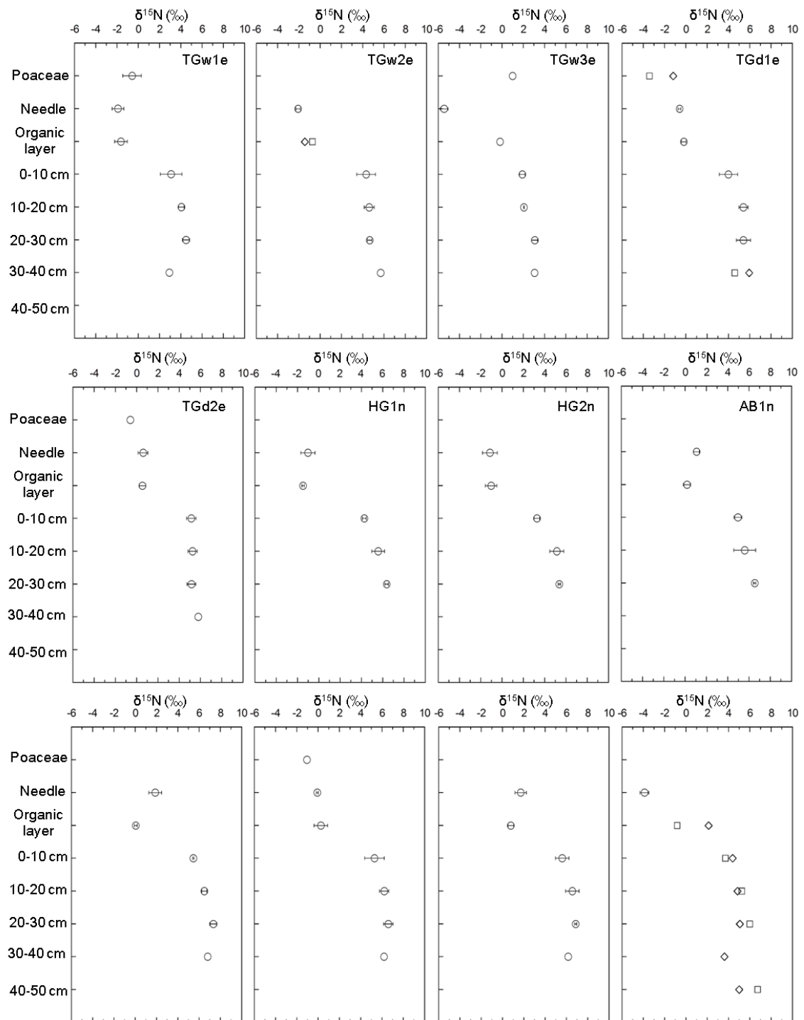
Figure 3.3. Vertical profiles of Poaceae, larch needle, organic layer, and bulk soil
