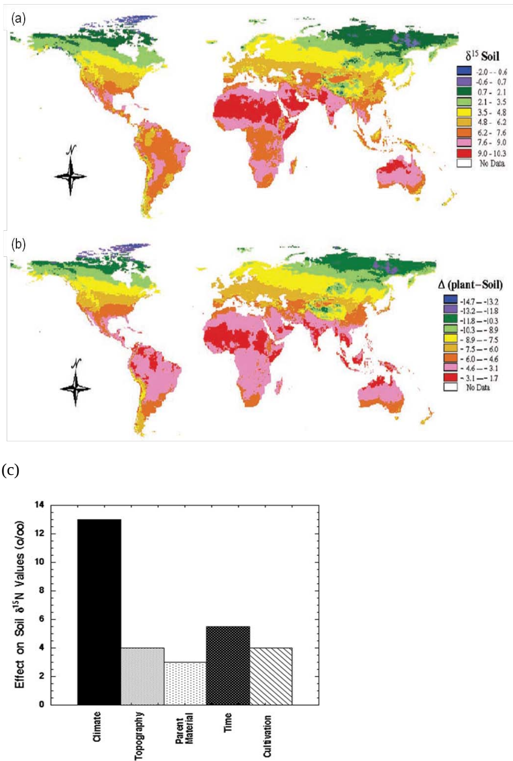
Figure 1.3. Geographical trends in soil \delta^{15}\text{N} (a), the difference between plant \delta^{15}\text{N} and soil \delta^{15}\text{N} (b), and estimated range in the effect of individual ecosystem state factor on the soil \delta^{15}\text{N} (c) in Amundson et al. (2003).
