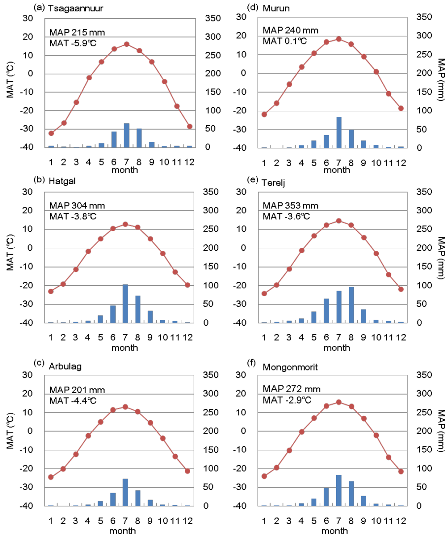
Figure 2.3. Monthly mean temperature (red line) and precipitation (blue bar) observed at meteorological station of study area: TG (a), HG (b), AB (c), MR (d), TR (e), and MM (f) in Mongolia for the period from 1993 to 2006. The latitude, longitude of each station are described above graph, and mean annual precipitation (MAP), mean annual temperature (MAT) are described in graph. The data was provided by meteorological station in institute of Meteorology and Hydrology, Mongolia.
