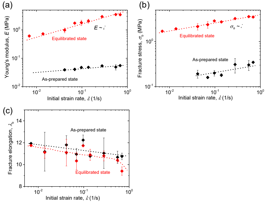
Figure 5. Initial strain rate \dot{\epsilon} dependence of Young's modulus E (a), fracture stress \sigma_b (b), and fracture elongation \lambda_b (c) of a polyampholyte hydrogel ( C_m=2.1 M) in its as-prepared and equilibrated state.
