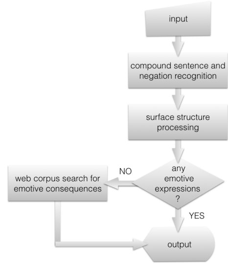
Figure 2: Sentiment analysis regarding compound sentences.
