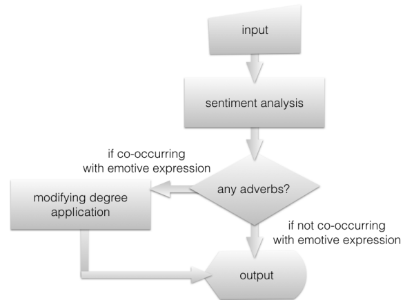
Figure 3: Applying modification degrees to adverbs.
