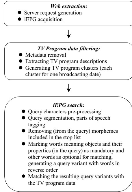
Figure 1. Input-output flow.
