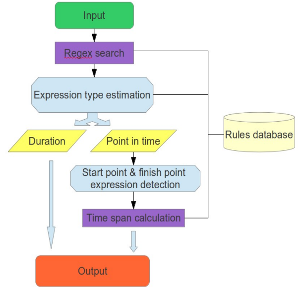
Figure 1: A-dur algorithm outline
