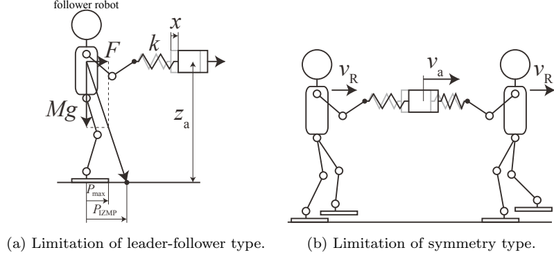
Figure 10. Limitation of moving velocity.
