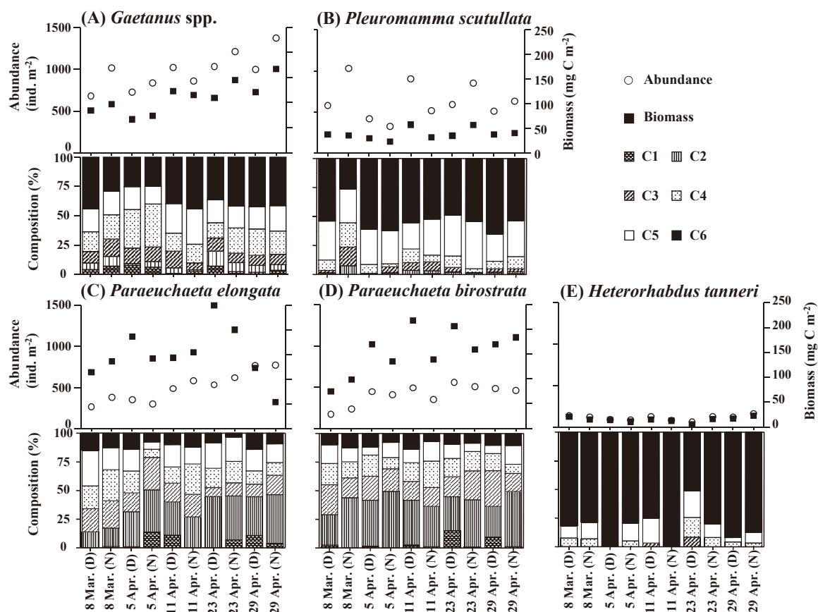
Fig. 10. Temporal changes in abundance, biomass and numerical copepodid stage composition of mesopelagic copepods, Gaetanus spp. (A), Pleuromamma scutellata (B), Paraeuchaeta elongata (C), P. birostrata (D) and Heterorhabdus tanneri (E), in the 0–1,000 m water column in the Oyashio region during March to April 2007. (D): day, (N): night.
