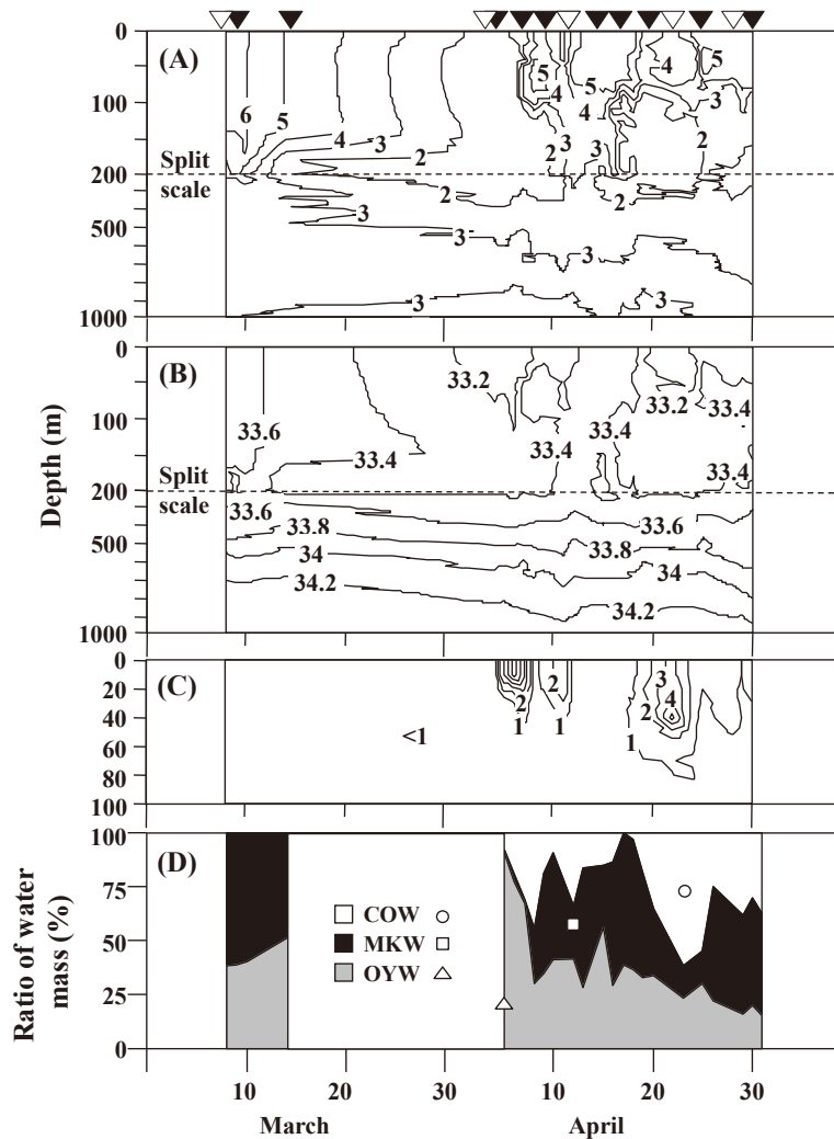
Fig. 4. Temporal changes in temperature (A, °C), salinity (B), chlorophyll a (C, mg m -3 ) and the ratio of water mass at 0–50 m water column (D, %) in the Oyashio region during 9 March to 1 May 2007. Data in D were from Kono and Sato (2010). Solid and open triangles at the top abscissa indicate sampling timings of the Bongo net and VMPS, respectively. Symbols in D indicate the dates that FRA-ROMS analysis was performed for each water mass (cf. Fig. 5). COW; coastal Oyashio water, MKW; modified Kuroshio water; OYW; Oyashio water.
