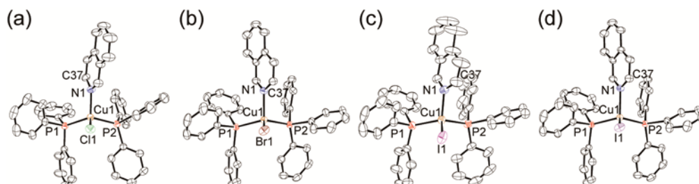
Figure 1. ORTEP drawings of 2-Cl (a), 2-Br (b), 2-I- \alpha (c) [14], and 2-I- \beta (d). Hydrogen atoms are omitted for clarity. Displacement parameters are drawn at the 50% probability level.
