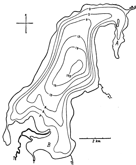
Fig. 1. Bathymetric map of Abasiri-ko.
