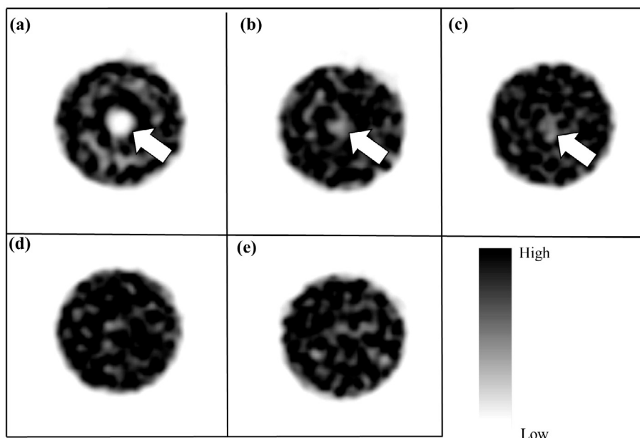
Fig. 1. For bed travels of (a) 0, (b) 30, (c) 60, (d) 90 and (e) 120 mm, reconstructed images of axial planes of the cylindrical phantom in helical SPECT scan are shown. The white arrows indicate remarkable artifacts.
