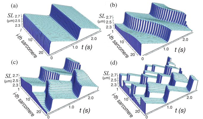
FIG. 2 (color). Examples showing typical spatiotemporal patterns of SL oscillations. (a), (b), (c), and (d) show, respectively, in-phase synchronization, traveling waves, disrupted traveling waves, and out-of-phase synchronization. The values of N and K used in each simulation are N = 24 and K = 0.01, 0.18, 0.7, 3.75 , respectively, and the values of the other parameters are indicated in the legend of Fig. 3. It is to be noted that the SPOC period largely depends on \eta_m as shown in Eq. (2), that is, the larger the value of \eta_m , the longer the SPOC period (see Fig. 8A in [14] for model simulation, and Figs. 3 and 4 in [3] for experimental results). The movies are shown in the Supplemental Material, Movie 2 [17].
