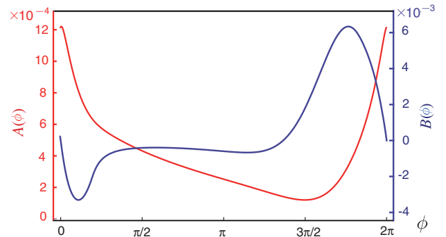
FIG. 4 (color). Phase-coupling functions obtained from Eq. (6). The parameters and the conditions are the same as in Fig. 3. A(\phi) (red) and B(\phi) (blue) are those for the global and local couplings, respectively.
