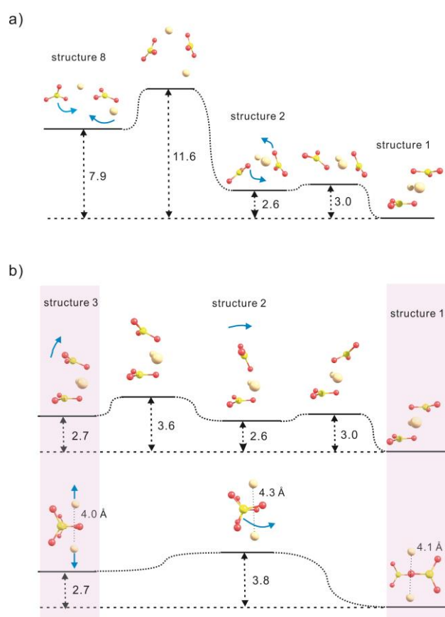
Fig. 2. Examples of the structural change process in additive-free \text{CaCO}_3 dimers. (a) Reaction path between Structure 8, which requires the most energy and Structure 1. (b) Reaction paths between Structures 3 and 1. Two types of reaction paths are shown: where the \text{CO}_3 ion ‘overhangs’ (above) and where \text{CO}_3 slides to another position (bottom). These two paths require almost the same activation energy. The relative energy of each equilibrium or transition structure based on the most stable structure is also shown in kcal/mol.
