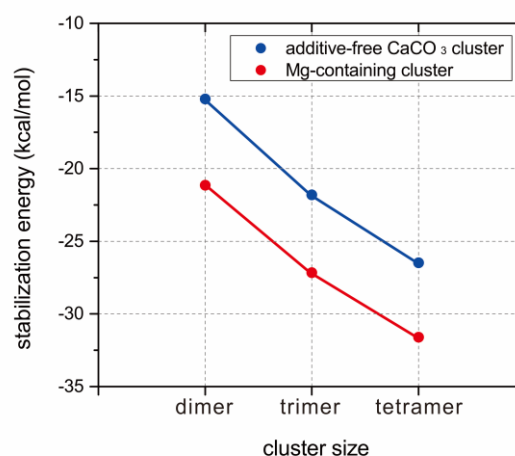
Fig. 9. Stabilization energy per monomer, varying with cluster size.
