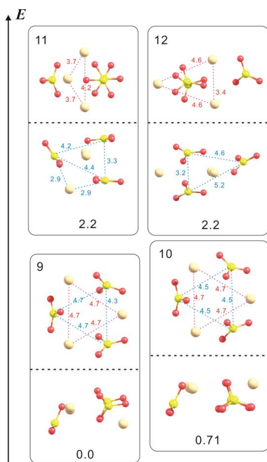
Fig. 4. Typical equilibrium structures of additive-free calcium carbonate trimers (\text{CaCO}_3)_3 . In this system, Structure 9 is the most stable. Dotted lines and their subscripts represent the interatomic distance in Å.
