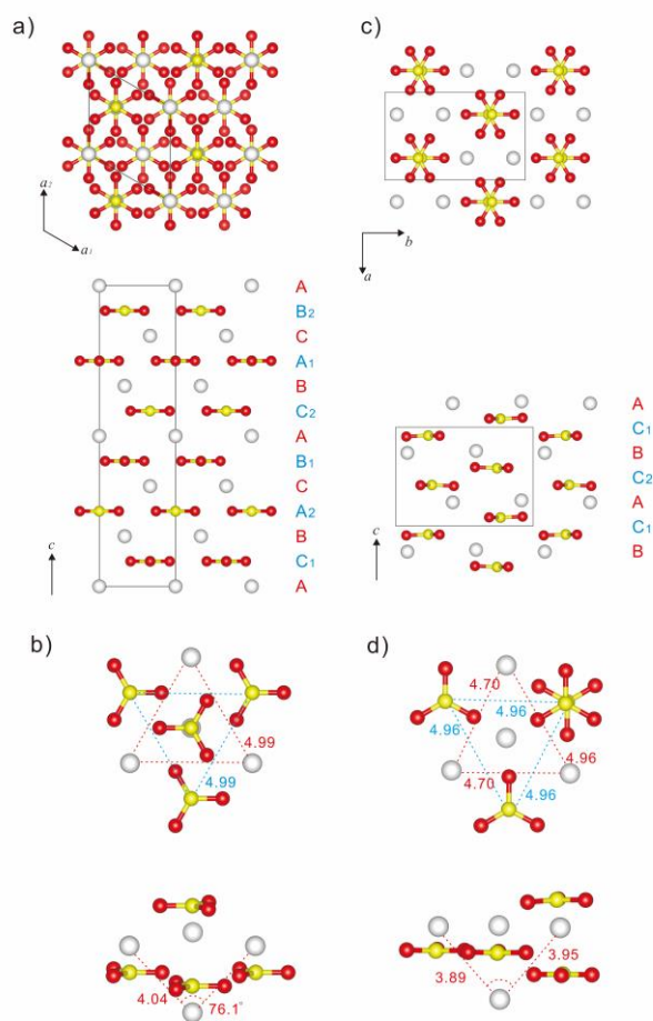
Fig. 8. (a) Bulk calcite structure, (b) local setting of Ca and CO 3 in a calcite structure, (c) bulk aragonite structure and (d) local setting of Ca and CO 3 in an aragonite structure. These figures were drawn with the VESTA program 36 .
