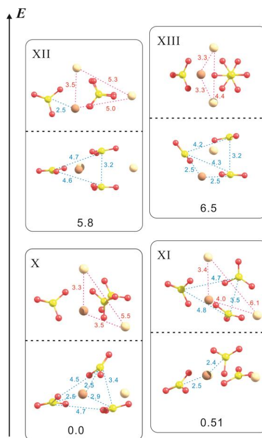
Fig. 5. Typical equilibrium structures of Mg-containing trimers, \text{Ca}_2\text{Mg}(\text{CO}_3)_3 . Dotted lines and their subscripts represent the interatomic distance in Å.
