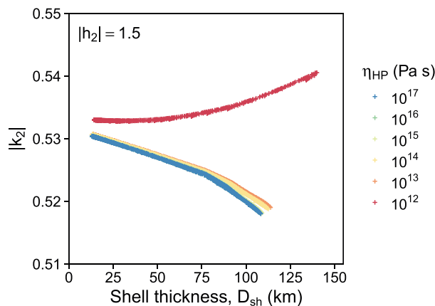
Figure 8. The absolute value of k_2 as a function of shell thickness ( D_{sh} ) for a given |h_2| . If |h_2| and \eta_{HP} is given, |k_2| is a good index for D_{sh} independent of \mu_{sh} and \eta_{ref} .
