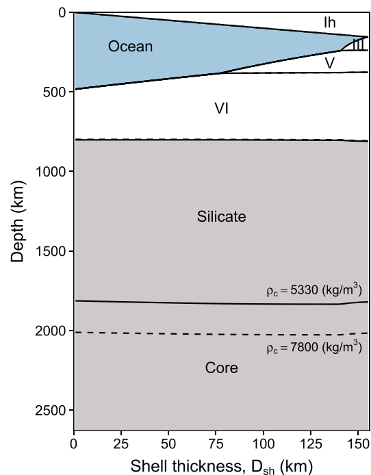
Figure 2. Our interior structure model for different shell thicknesses ( D_{\text{sh}} ). Solid and dashed curves show results for the core density \rho_c of 5330 and 7800 \text{kg m}^{-3} , respectively. The difference in \rho_c strongly affects the radius of the core. See Table 1 for parameters adopted.
