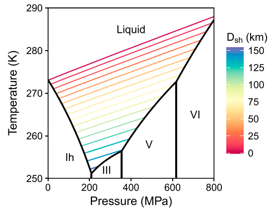
Figure 1. Phase diagram of \text{H}_2\text{O} [Choukroun and Grasset, 2010]. Colored lines show temperature profiles of our models for different shell thicknesses ( D_{\text{sh}} ). A thinner shell has a higher ocean temperature, leading to a thicker ocean.
