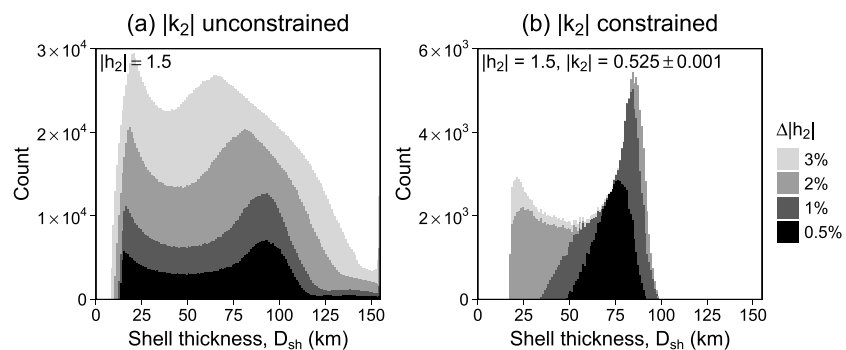
Figure 9. Histogram of the thickness of the ice Ih shell ( D_{sh} ) for a given |h_2| with different errors. Results under conditions where |k_2| is (a) unconstrained and (b) constrained. The increase in the precision of |h_2| decreases the uncertainty in the shell thickness only if |k_2| is constrained.
