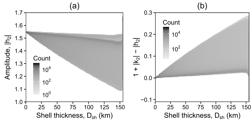
Figure 7. Two-dimensional histogram of (a) tidal amplitude ( |h_2| ) and of (b) a linear combination of Love numbers as functions of shell thickness ( D_{sh} ). A thin and a thick shell have small and large variations in |h_2| and 1 + |k_2| - |h_2| .
