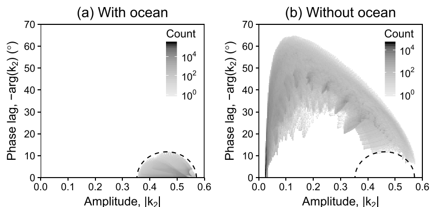
Figure 5. Two-dimensional histogram of the gravitational tidal response for (a) cases with a subsurface ocean and for (b) cases without a subsurface ocean. The horizontal and vertical axes represent the absolute value and the argument of the potential Love number ( k_2 ), respectively. The dashed oval represents the distribution of solutions for cases with an ocean.
