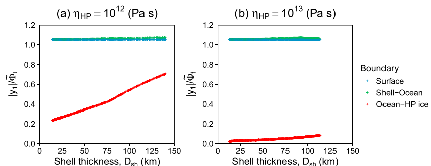
Figure B1. Amplitude of vertical displacement |y_1| normalized by tidal potential \Phi_t . Results for three different depths (i.e., the surface, the base of the ice Ih shell, and the top of the HP ice layer) are shown.
