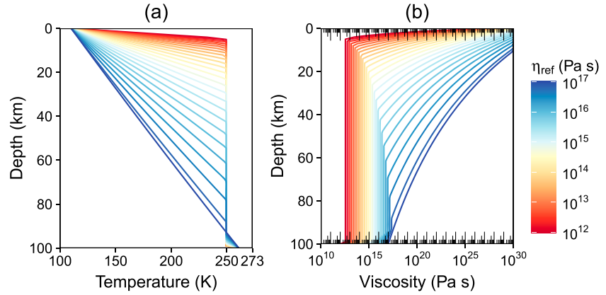
Figure 3. (a) Temperature and (b) viscosity profiles of the top ice Ih shell for different reference viscosities ( \eta_{\text{ref}} ). Results for shell thickness D_{\text{sh}} = 100 km are shown. Because of the thick shell, thermal convection occurs for most cases, leading to a constant temperature and viscosity region.
