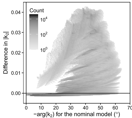
Figure A1. Difference in |k_2| between our nominal model (i.e., \rho_m = 3222 \text{ kg m}^{-3} ) and models with \rho_m = 3022 \text{ kg m}^{-3} . Results for cases without a subsurface ocean are shown. A large difference can be found only for cases with a large phase lag.
