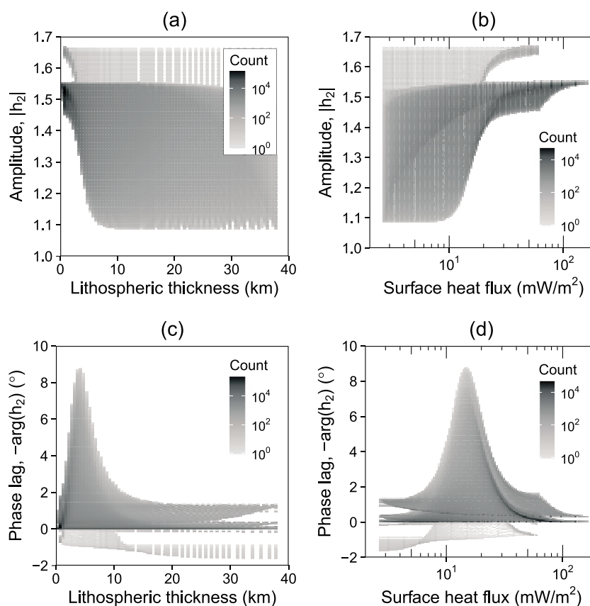
Figure 10. Two-dimensional histogram of (a) lithospheric thickness versus tidal amplitude, (b) surface heat flux versus tidal amplitude, (c) lithospheric thickness versus phase lag, and (d) surface heat flux versus phase lag.
