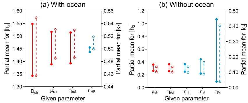
Figure 6. Partial mean values of the absolute value of Love numbers for (a) cases with a subsurface ocean and for (b) cases without a subsurface ocean. Results for |h_2| are shown using solid lines and closed circles, while those for |k_2| are shown using dashed lines and open circles. Red and blue lines and symbols are variables for the ice Ih shell and for high-pressure ice layers, respectively. The factor that leads to the largest variation in partial means is D_{sh} for Figure 6a and \eta_{VI} for Figure 6b.
