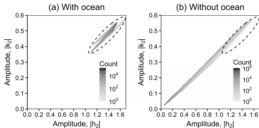
Figure 4. Two-dimensional histogram of the tidal amplitude for (a) cases with a subsurface ocean and for (b) cases without a subsurface ocean. The horizontal and vertical axes represent the absolute value of the displacement Love number ( h_2 ) and that of the potential Love number ( k_2 ), respectively. The dashed oval represents the distribution of solutions for cases with an ocean.
