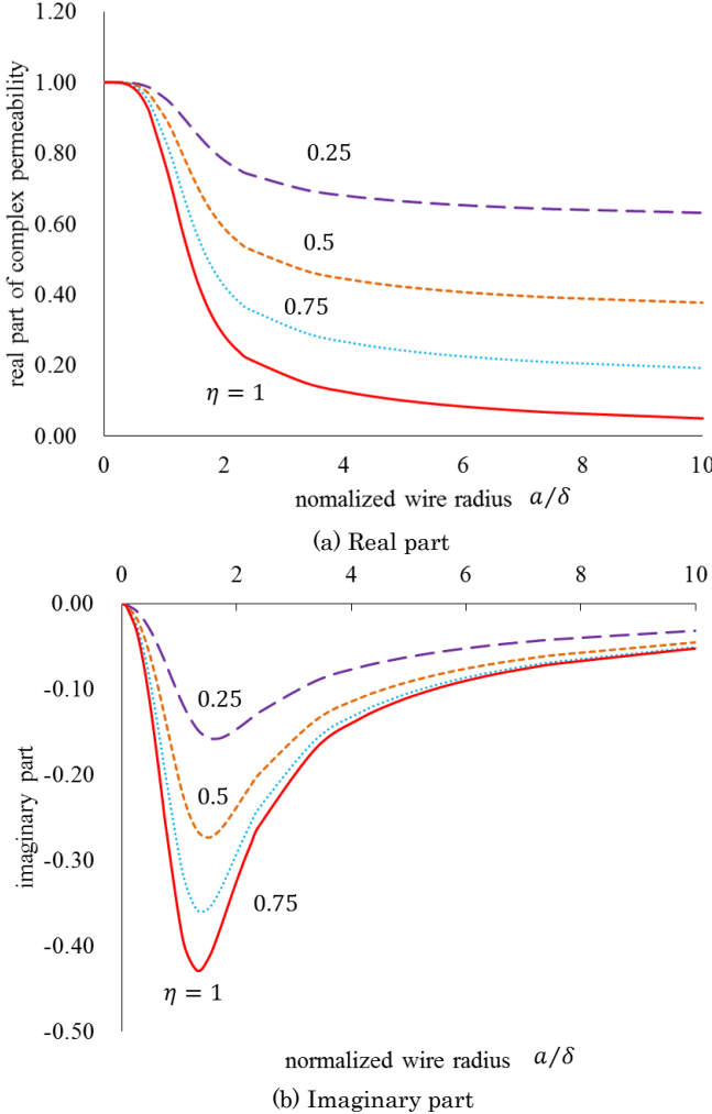
Fig.2 Dependence of homogenized permeability \langle \dot{\mu}_r \rangle on normalized radius a/\delta , where \delta denotes skin depth.
