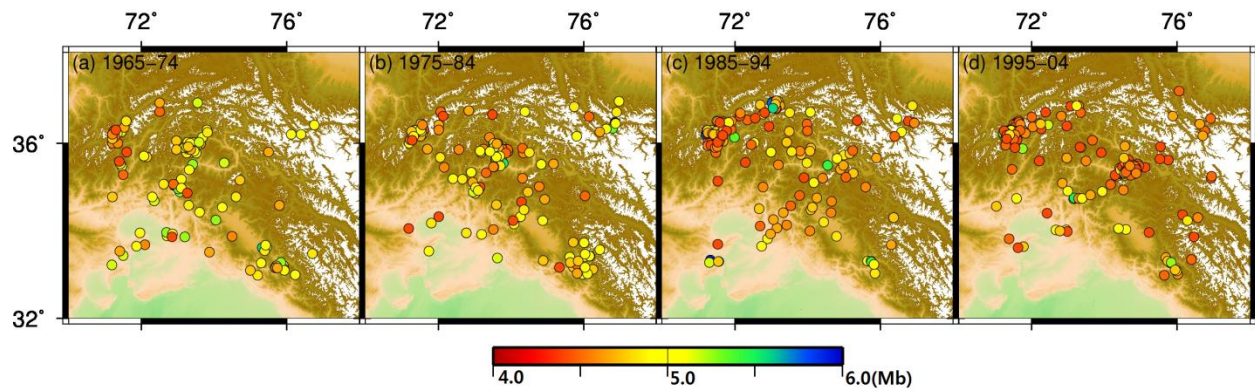
Fig. 5 Epicentral plot for different magnitudes in the corresponding decades.
