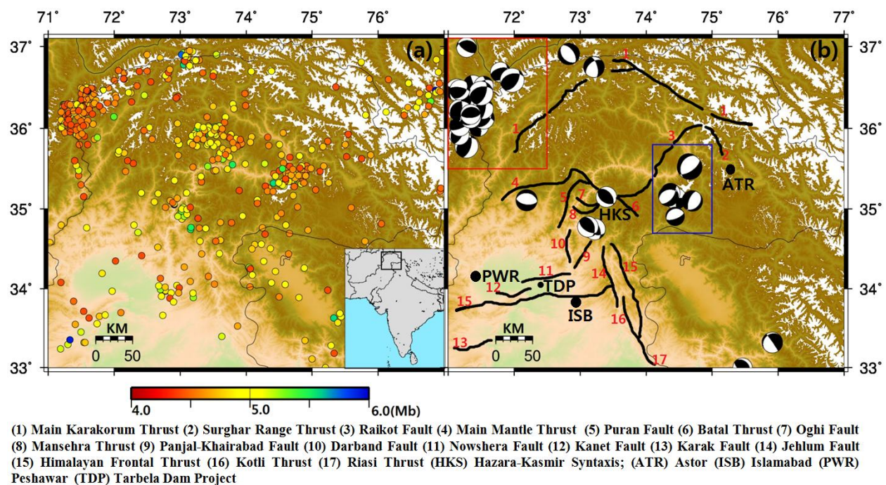
Fig. 1 (a) The historical seismicity and the some important active faults of northern Pakistan. The colored dots, plotted by using Pakistan Meteorological data, indicate the magnitude and location of the earthquakes. (b) The faults are from Lisa et al. (2007). The beach balls are derived from Global Centeroid Moment Tensor (GCMT) data.
