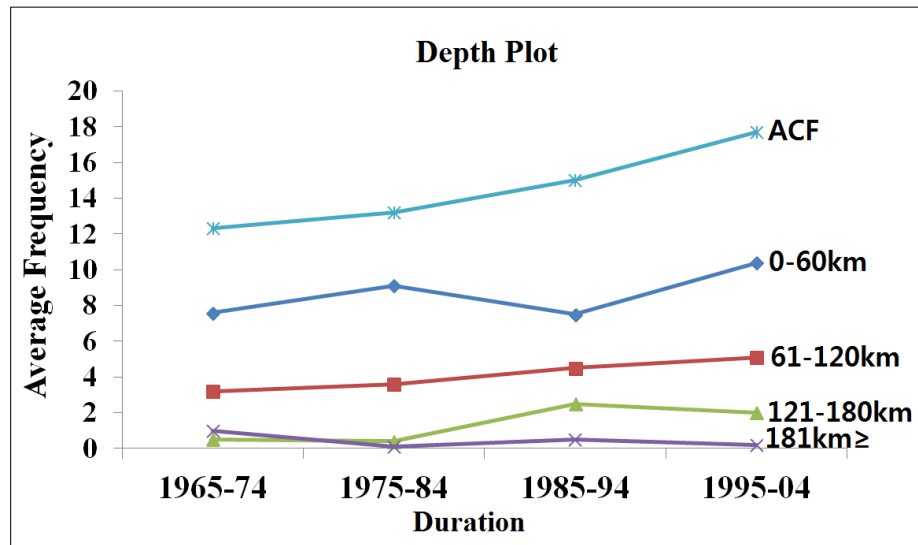
Fig. 6 Depth plot. ACF is Average Cumulative Frequency
