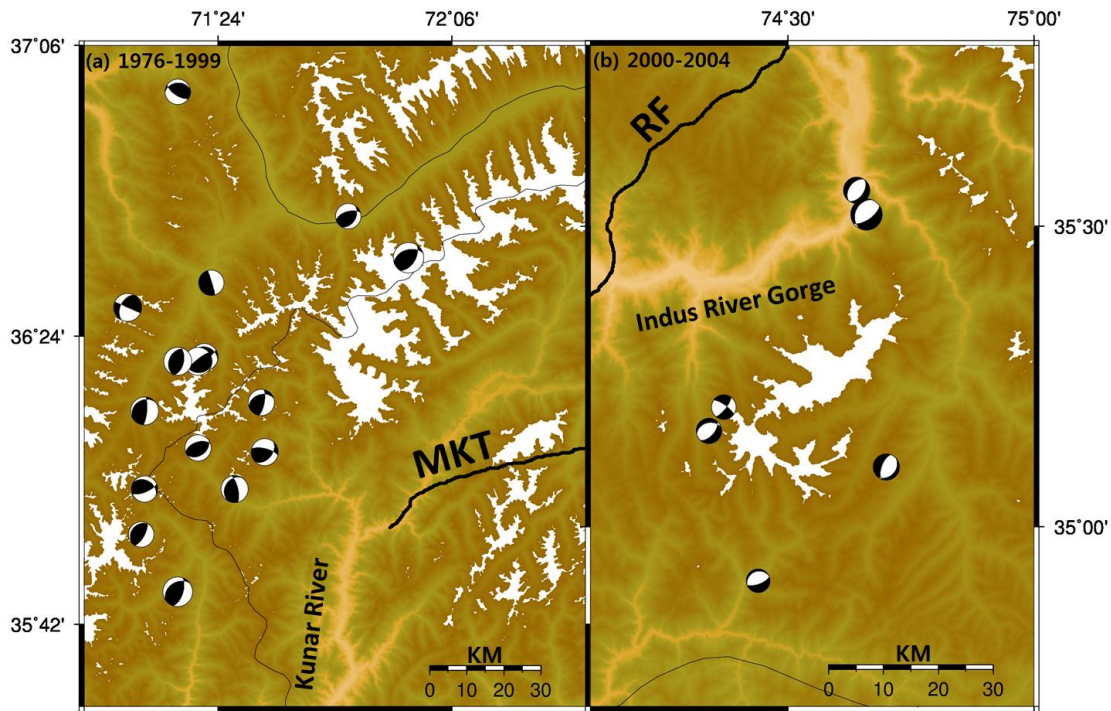
Fig. 3 Magnified view of the FMS clustered areas. MKT is Main Karakorum Thrust and RF is Raikot Fault
