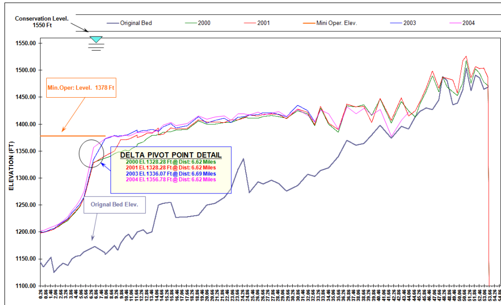
Fig. 2 Sediment Longitudinal Profile of Tarbela Dam. The horizontal axis shows the distance in miles (Tarbela Dam Project 2010).
