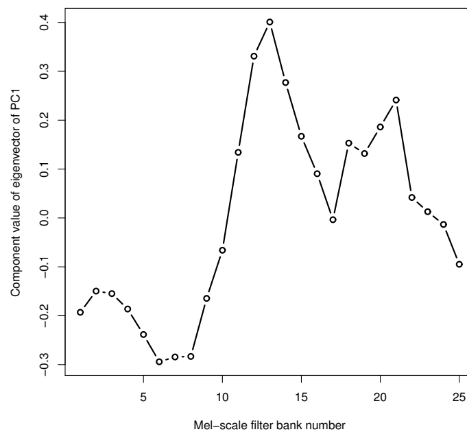
FIGURE 3.11: Eigenvector of the first principal component for /a/ uttered by a male speaker [29].
