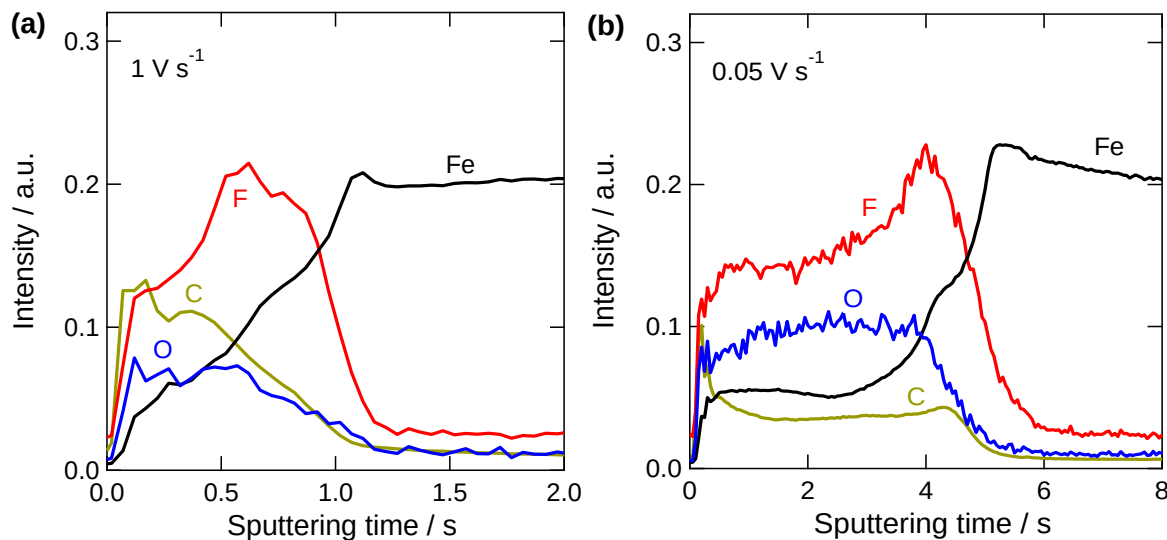
Figure 4.4 GDOES depth profile analysis of anodic films formed on the iron sheet at a sweep rate of (a) 1 V s -1 (b) 0.05 V s -1 in the EG electrolyte containing 0.1 mol dm -3 ammonium fluoride and 0.1 mol dm -3 H 2 O at 273 K.
