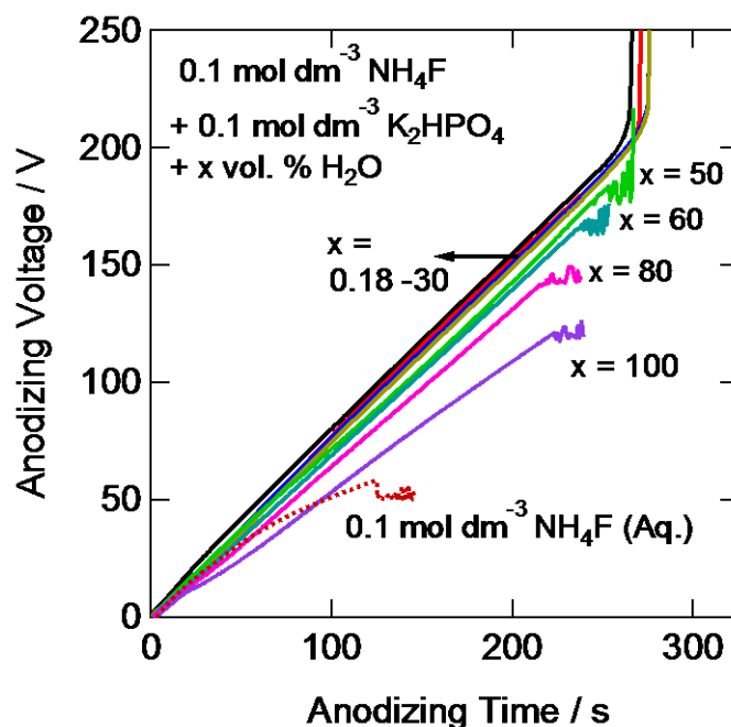
Figure 5.1 Voltage-time responses of the magnetron-sputtered magnesium films during anodizing at a current density of 10 \text{ A m}^{-2} in the EG- \text{H}_2\text{O} electrolytes containing 0.1 \text{ mol dm}^{-3} ammonium fluoride, 0.1 \text{ mol dm}^{-3} dipotassium hydrogen phosphate and x \text{ vol. \% H}_2\text{O} and an aqueous electrolyte containing 0.1 \text{ mol dm}^{-3} ammonium fluoride at 293 \text{ K} .
