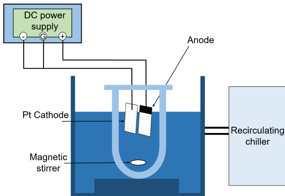
Figure 2.4 Schematic illustration of the anodizing apparatus used in this study, indicating two electrodes anodizing cell in a large cooling vessel and chiller.
