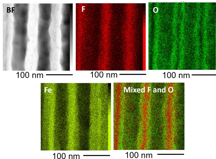
Figure 3.25 Bright field image and corresponding EDS maps of the middle region of FIB-treated anodic film formed on iron at 40 V in the ethylene glycol electrolyte containing 1.5 mol dm -3 water and 0.1 mol dm -3 ammonium fluoride at 293 K.
