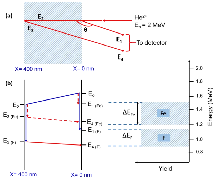
Figure 2.7 (a) Schematic illustration of geometry of scattering and notation of energies at front and back surfaces of a 400 nm-thin iron fluoride film and (b) change in the energy of \text{He}^{2+} ions during traveling a 400 nm-thin iron fluoride thin film.
