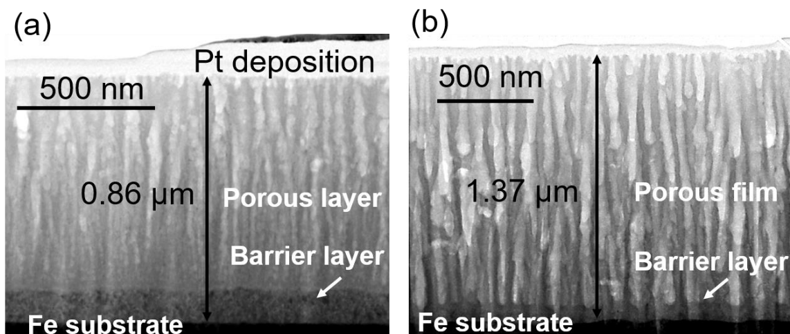
Figure 3.27 Transmission electron micrographs of FIB-treated anodic films potentiodynamically formed on iron at 50 V in the ethylene glycol electrolyte containing 0.1 mol \text{dm}^{-3} ammonium fluoride and (a) 0.1 (b) 0.5 mol \text{dm}^{-3} water at 293 K.
