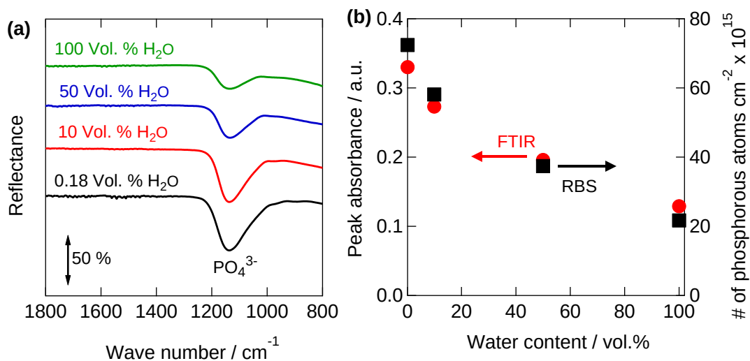
Figure 5.10 (a) FTIR spectra of the magnetron-sputtered magnesium films anodized to 100 V at 10 A m -2 in the EG-H 2 O electrolytes containing 0.1 mol dm -3 ammonium fluoride, 0.1 mol dm -3 dipotassium hydrogen phosphate and various concentrations of H 2 O and (b) Change in the peak absorbance and the number of phosphorus atoms in the anodic films with comparison of reduction in number of phosphorous atoms and peak absorption by RBS and FTIR respectively in the same electrolytes.
