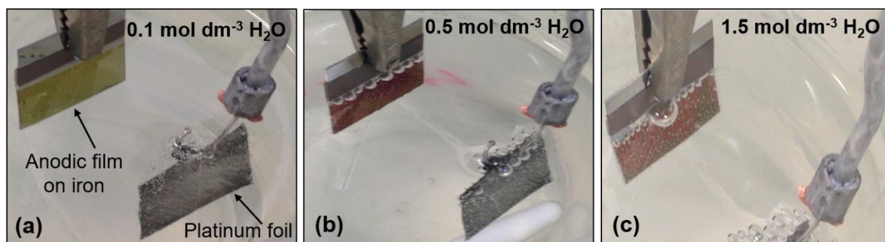
Figure 3.5 Images of gas evolution during anodizing of iron anodized at 50 V for 15 min in ethylene glycol electrolyte containing 0.1 mol dm -3 ammonium fluoride and (a) 0.1, (b) 0.5, and (c) 1.5 mol dm -3 water at 293 K.
