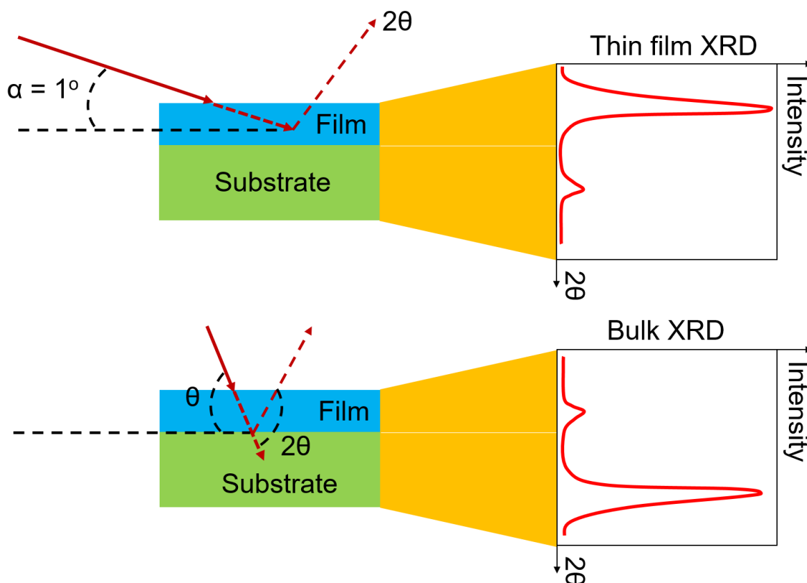
Figure 2.8 Schematic diagram illustrating the glazing incidence and bulk modes of X-ray diffraction measurements.
