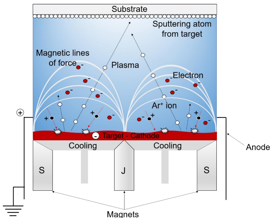
Figure 2.3 Diagram showing the magnetron sputtering [1].
