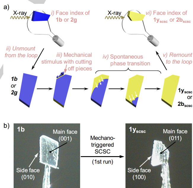
Figure 5. a) Schematic representation of the procedure used for the face index experiments of 1 and 2 . b) Photographs of the single crystals of 1b and 1y scsc (taken under room light) which were used for the face indexing experiments through the mechano-triggered SCSC phase transitions (1st run). See the Supporting Information for the photographs of 2nd and 3rd run.
