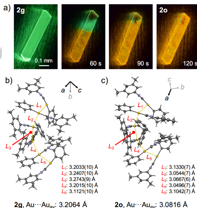
Figure 12. a) A series of photographs showing the thermal SCSC phase transition of 2g to 2o at 55°C. The photographs were taken under the ambient conditions and 365-nm illumination. ORTEP representations of the hexamer unit of b) 2g and c) 2o showing the multiple intermolecular aurophilic interactions.
