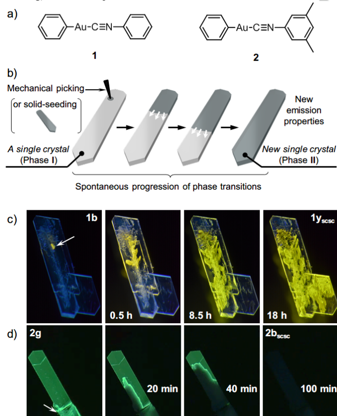
Figure 1. a) Structures of 1 and 2 . b) Schematic representation of the SCSC phase transition, triggered by mechanical picking and solid-seeding, that is accompanied by a photoluminescence color change. A series of photographs following the mechano-
