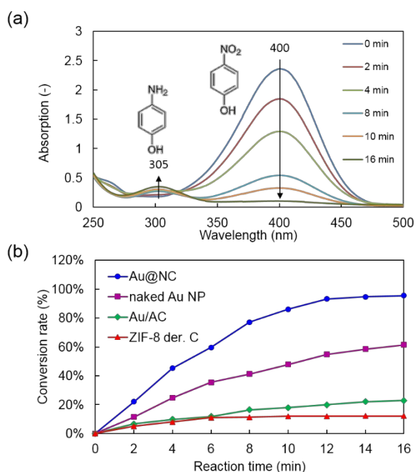
Figure 4. (a) UV-Vis spectroscopy for the reduction of 4-nitrophenol catalyzed by Au@NC at different time periods. (b) The reduction of 4-nitrophenol by ZIF-8 derived carbon, Au-loaded activated carbon (Au/AC), naked Au nanoparticles derived from Au@NC and Au@NC.
