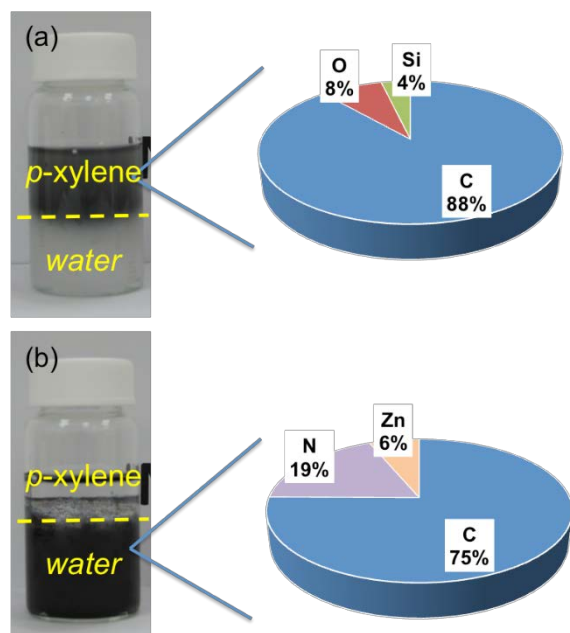
Figure 5. The hydro compatibility of ZIF-8 derived carbon (C) and activated carbon (AC). (a) Au/AC suspended and (b) Au@NC suspended mixture solution. The composition of carbon based structure was analyzed with XPS.
