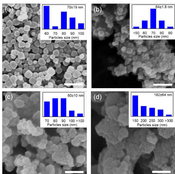
Figure 1. The SEM images of \text{AuCl}_4^-/\text{ZIF-8} with different molar ratio of Au to Zn. (a) 0:1, (b) 0.01:1, (c) 0.1:1 and (d) 0.2:1. The scale bar is 250 nm. The particle size distribution was calculated with TEM images ( n > 100 ).
