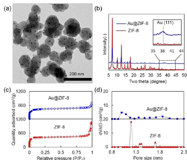
Figure 2. (a) A TEM image of Au@ZIF-8. (b) XRD Patterns of Au@ZIF-8 and ZIF-8. (c) \text{N}_2 adsorption/desorption isotherms of Au@ZIF-8 and ZIF-8. (d) The corresponding pore size distribution of Au@ZIF-8 and ZIF-8.
