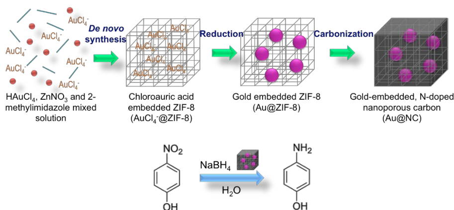
Scheme 1. De novo synthesis of Au nanoparticles-embedded, nitrogen-doped nanoporous carbon particles for reduction of 4-nitrophenol.
