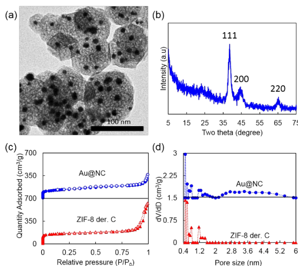
d) N 2 adsorption/desorption and pore size distribution, respectively, of Au@NC and ZIF-8 derived carbon.
