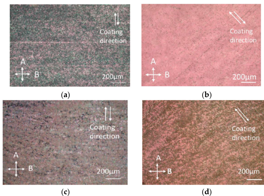
Figure 2. Microphotographs taken after slit coating. Host NLC used was MLC-14100-000: (a) without doping and with the coating direction parallel to the analyzer; (b) without doping and with the coating direction 45^\circ with respect to the analyzer; (c) with nanoparticle doping and the coating direction parallel to the analyzer; and (d) with nanoparticle doping and the coating direction 45^\circ with respect to the analyzer.
