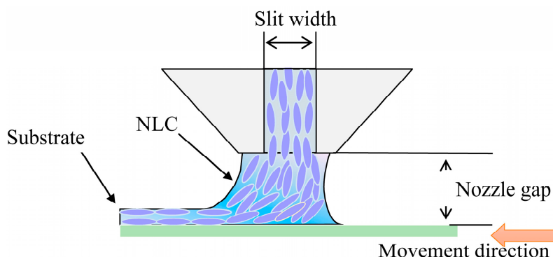
Figure 1. Schematic diagram of the slit coater.
