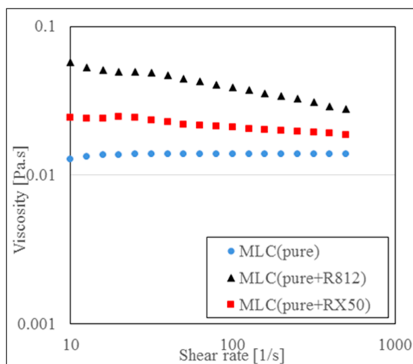
Figure 3. The shear rate dependence of the viscosity for MLC-14100-000 systems with and without nanoparticles, R812 and RX50.
