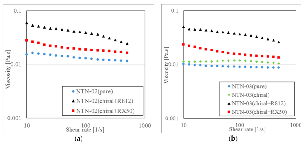
Figure 4. The shear rate dependence of the viscosity for NTN-02 (a) and NTN-03 (b) with and without nanoparticles, R812 and RX50.
