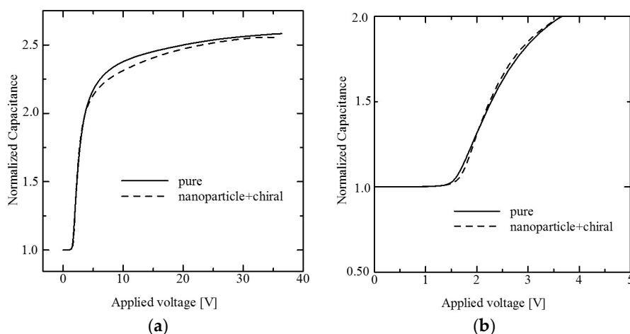
Figure 6. (a) Dependence of the normalized NLC cell capacitance on the applied voltage with and without doping with R-812 and (b) enlarged view of the region of (a) around the threshold voltage.
