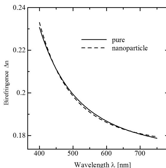
Figure 5. Birefringence wavelength dispersion values, \Delta n , with and without doping with R-812.
