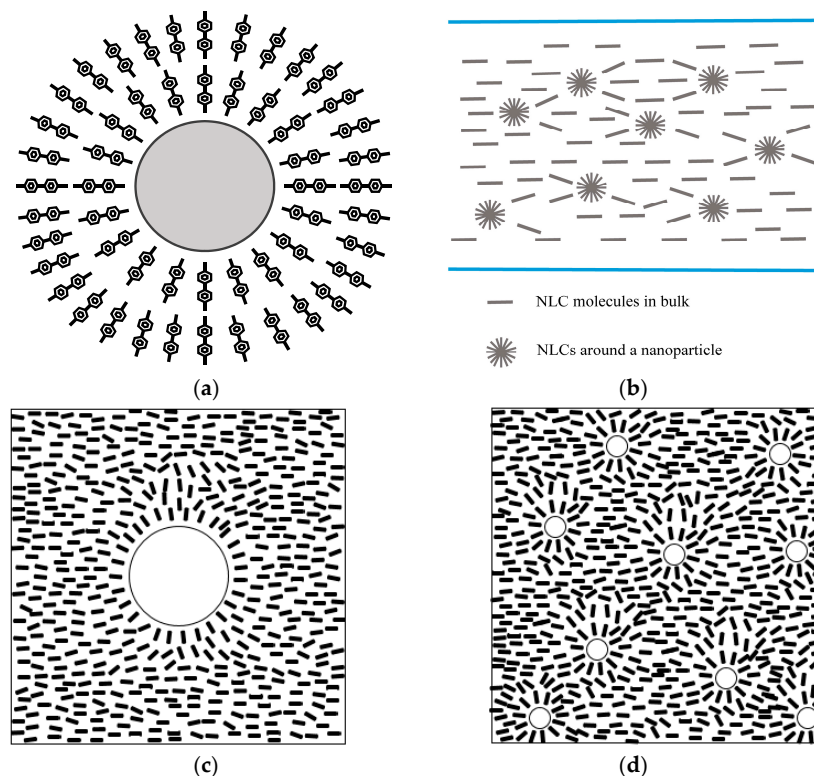
Figure 7. (a) NLC alignment around a single nanoparticle; (b) the bulk NLC/nanoparticle mixture; (c) NLC alignment around a 40 nm RX-50 nanoparticle; and (d) NLC alignment around 7 nm R-812 nanoparticles, applying the same mass of nanoparticles as in the case of (c).
