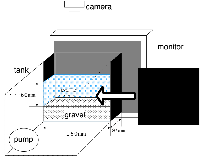
Figure 2: Experimental set-up
