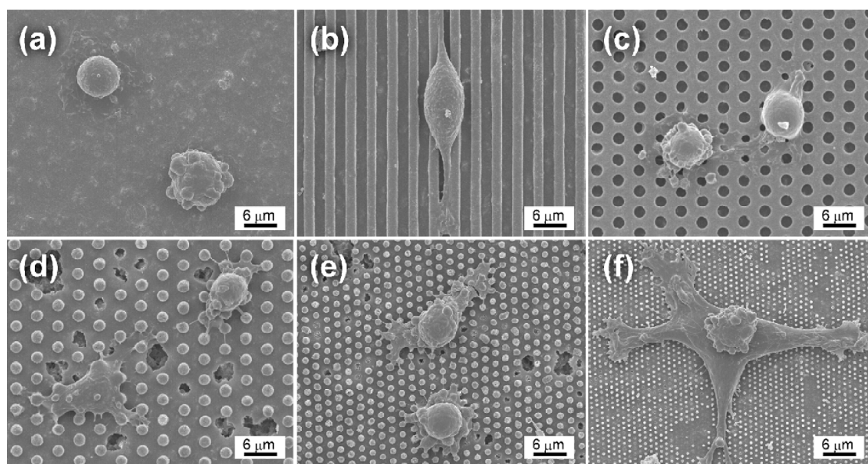
Fig. 5 SEM images of attached Saos-2 cells on the micro-/submicro-patterned apatite after 1 h of incubation. (a) Planar, (b) 2\text{-}\mu\text{m} grooves, (c) 2\text{-}\mu\text{m} holes, (d) 2\text{-}\mu\text{m} pillars, (e) 1\text{-}\mu\text{m} pillars, and (f) 0.5\text{-}\mu\text{m} pillars.
