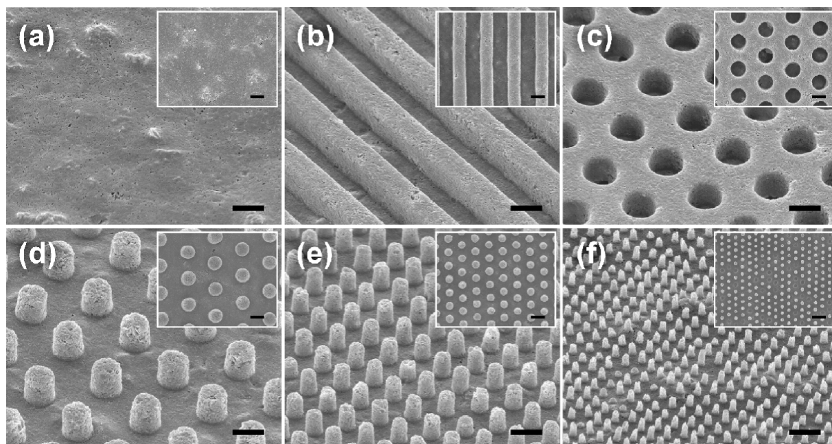
Fig. 2 SEM images of the surface of patterned apatite at an angle of 45 degrees. Insets show top-view images of the surface of the pattern. (a) Planar, (b) 2-μm grooves, (c) 2-μm holes, (d) 2-μm pillars, (e) 1-μm pillars, and (f) 0.5-μm pillars. Scale bar: 2 μm.
