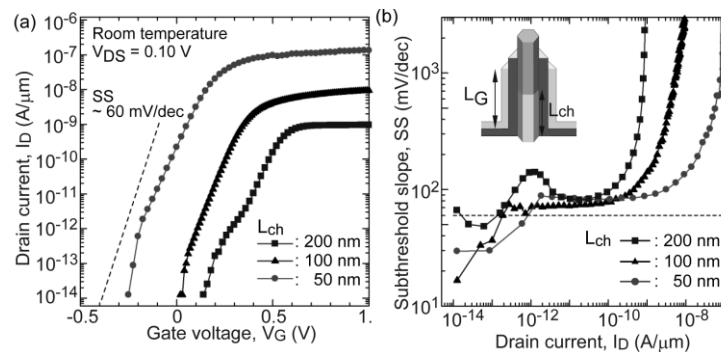
Figure 5. (a) Transfer curves for different values of L_{\text{ch}} . V_{\text{DS}} = 0.10 \text{ V} at RT in the dark. The dashed line plots the theoretical limit of carrier thermal diffusion ( \text{SS} = 60 \text{ mV/decade} ). (b) SS as a function of drain current. The dashed line shows the limit of MOSFETs ( = 60 \text{ mV/decade} ). The inset illustrates the NW-channel. Note that the device was different from that of Figure 4.
