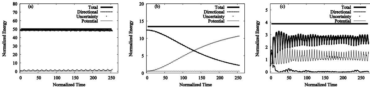
Fig. 4. Time evolution of normalized energies for 40 gyrations. (a) Normalized initial speed v_0 = 10 and normalized initial energy, E = 50.254 . (b) Normalized initial speed v_0 = 5 and normalized initial energy, E = 13.458 . (c) Normalized initial speed v_0 = 1 and normalized initial energy, E = 3.892 .
