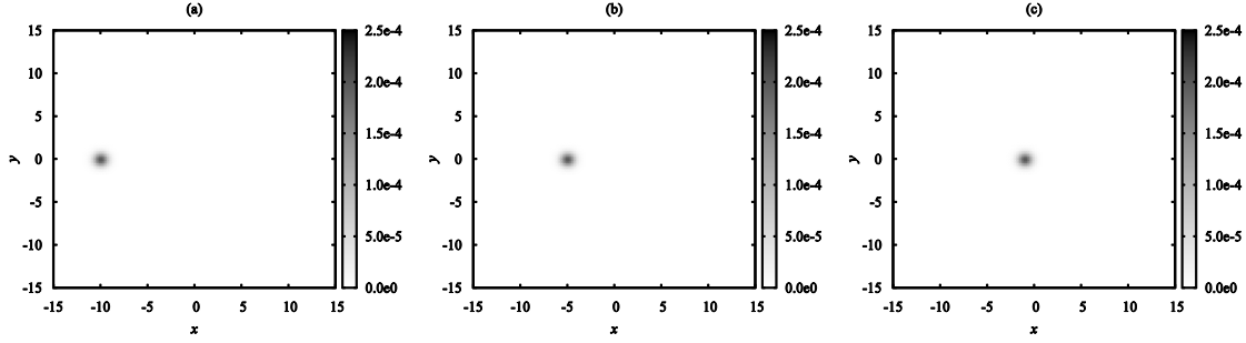
Fig. 2. Initial condition t = 0 of probability density function (PDF) of a single charged particle, in the presence of a fixed field particle at the origin. (a) Normalized initial speed v_0 = 10 . (b) Normalized initial speed v_0 = 5 . (c) Normalized initial speed v_0 = 1 .
