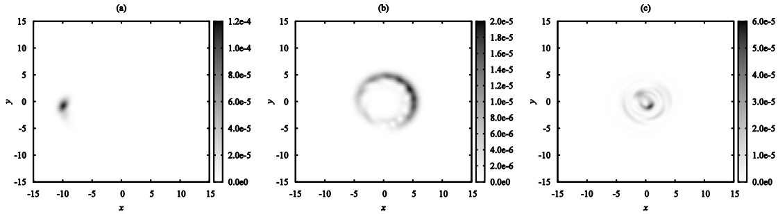
Fig. 3. The PDF of a single charged particle, in the presence of a fixed field particle at the origin, after 40 gyrations. (a) Normalized initial speed v_0 = 10 . (b) Normalized initial speed v_0 = 5 . (c) Normalized initial speed v_0 = 1 .
