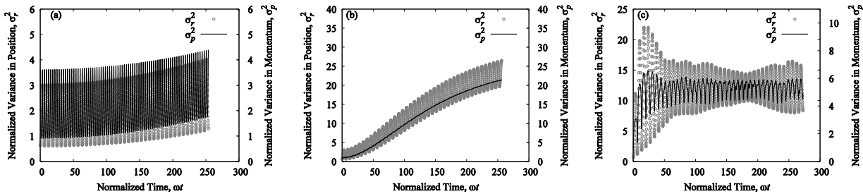
Fig. 5. Normalized variance in position \sigma_r^2 and total momentum \sigma_p^2 , for 40 gyrations. (a) Normalized initial speed v_0 = 10 . (b) Normalized initial speed v_0 = 5 . (c) Normalized initial speed v_0 = 1 .
