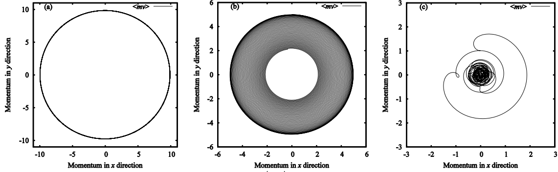
Fig. 6. Normalized expectation values of momentum \mathbf{p} = \langle m\mathbf{v} \rangle after 40 gyrations. (a) Normalized initial speed v_0 = 10 and normalized initial momentum (mu_0, mv_0) = (0, 10) . (b) Normalized initial speed v_0 = 5 and normalized initial momentum (mu_0, mv_0) = (0, 5) . (c) Normalized initial speed v_0 = 1 and normalized initial momentum (mu_0, mv_0) = (0, 1) .
