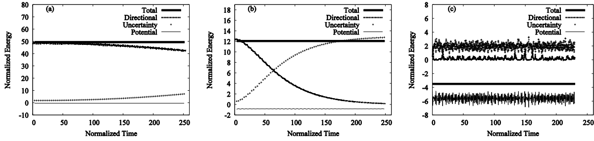
Fig. 8. Time evolution of normalized energy for 40 gyrations. (a) Normalized initial speed v_0 = 10 and initial normalized energy, E = 49.592 . (b) v_0 = 5 with E = 12.119 . (c) v_0 = 1 with E = -3.457 .
