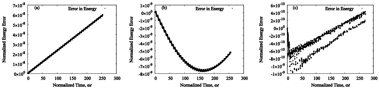
Fig. 1. Time evolution of relative errors in energy, in the presence of a fixed field particle at the origin. (a) Normalized initial speed v_0 = 10 . (b) Normalized initial speed v_0 = 5 . (c) Normalized initial speed v_0 = 1 .
