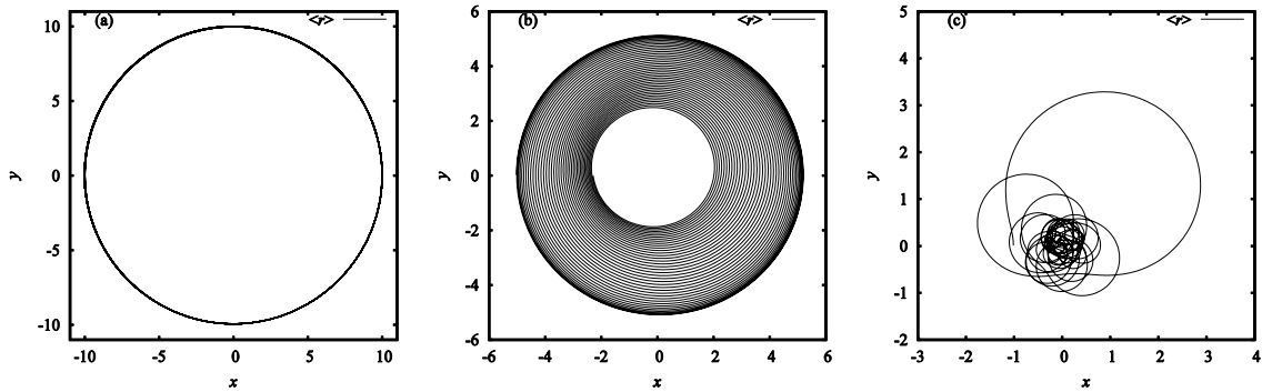
Fig. 7. Normalized expectation position \langle \mathbf{r} \rangle after 40 gyrations. (a) Normalized initial speed v_0 = 10 and initial position (-10, 0) . (b) Normalized initial speed v_0 = 5 and initial position (-5, 0) . (c) Normalized initial speed v_0 = 1 and initial position (-1, 0) .
