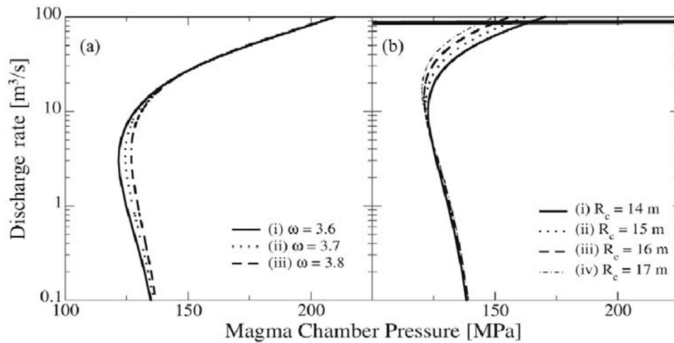
Fig. 5. Relation between the magma chamber pressure and volumetric discharge rate in the steady solutions without fragmentation. (a) Variations with the permeability exponent, \omega . Other parameters are fixed as R_c = 10 m, T = 980^\circ\text{C} , n_0 = 4.0 wt%, L = 6 km, E_w = 0 . (b) Variations with conduit radius, R_c . Other parameters are fixed as \omega = 3.8 , T = 980^\circ\text{C} , n_0 = 4.0 wt%, L = 6 km, E_w = 0 . Dashed line indicates the observed discharge rate ( 87 \text{ m}^3/\text{s} ) for the lava extrusion stage.
