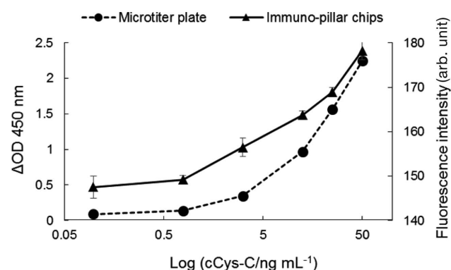
Fig. 3 Standard curves for cCys-C using the immuno-pillar chips (solid line with right Y-axis) and microtiter plate (dashed line with left Y-axis).
