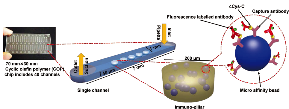
Fig. 2 Schematic of cCys-C assay in a channel of the immuno-pillar chips.
