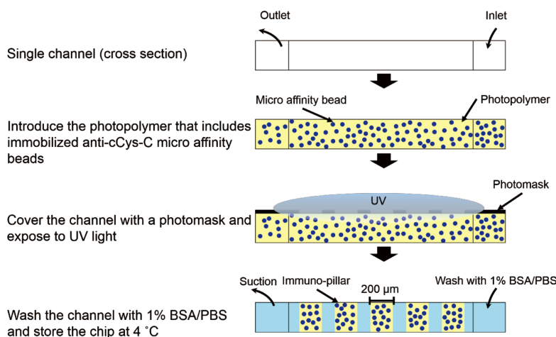
Fig. 1 Fabrication steps for the photopolymerized micro immuno-pillars.
