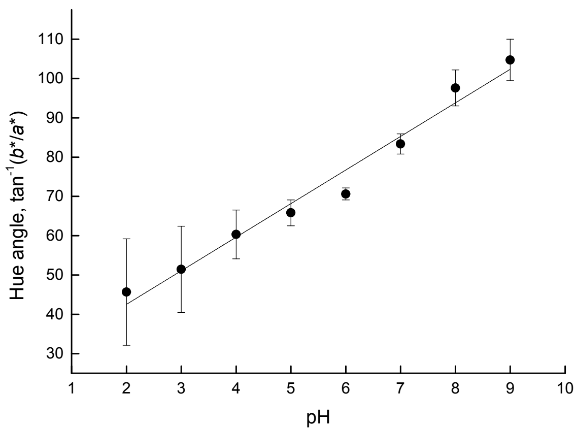
Fig. S5 Plot of \tan^{-1}(b^*/a^*) at various pH values in CIE L^*a^*b^* color system
