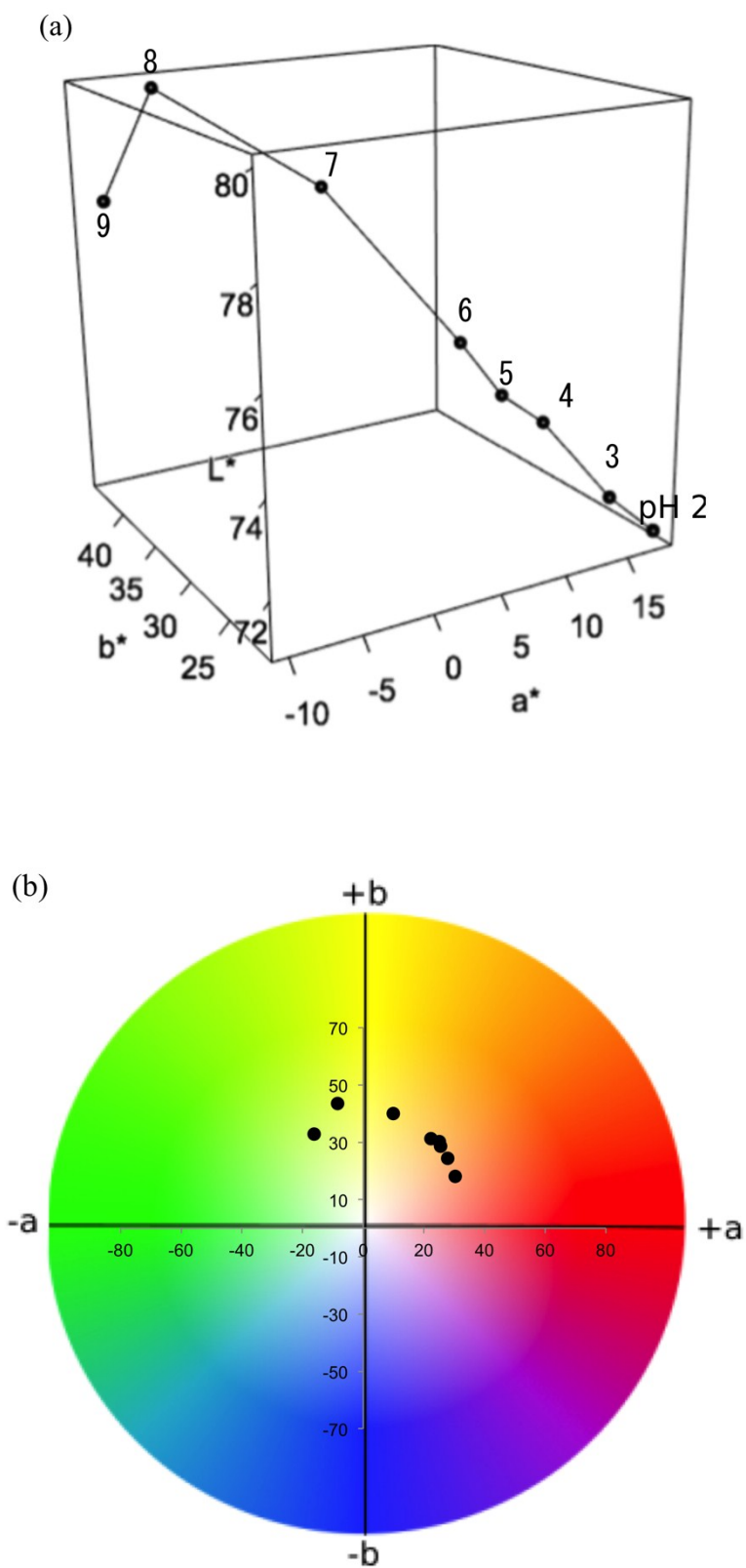
Fig. S3 (a) 3D and (b) 2D plot of various pH values in CIE L^*a^*b^* color system.
