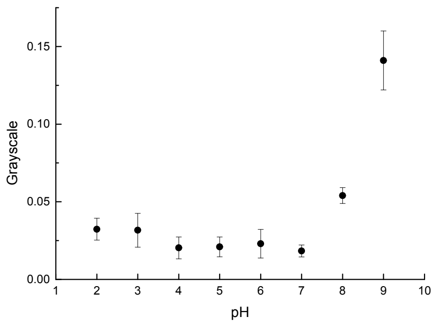
Fig. S2 Plot of grayscale against pH value.
