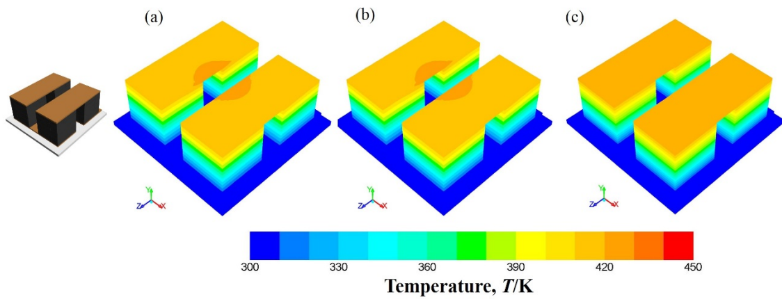
Fig.6 Temperature profiles when the maximum output powers generated. (a), (b) and (c) correspond to the model I, II and III, respectively.
