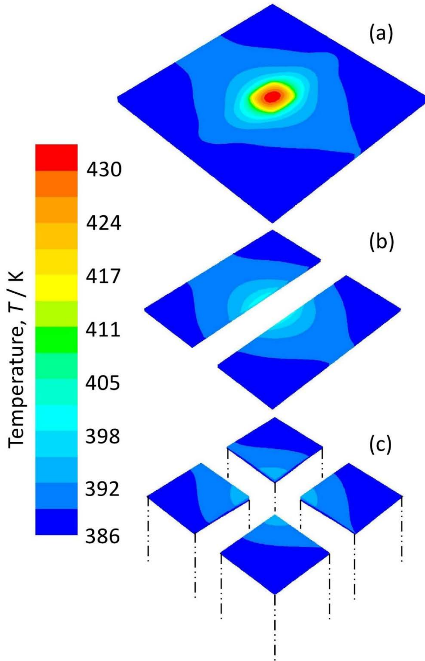
430 Fig.7 Temperature distributions on (a) top surface of alumina plate, (b) upper surface of 431 electrodes, and (c) upper surfaces of TE elements, when the maximum output power generated 432 at the model I.
