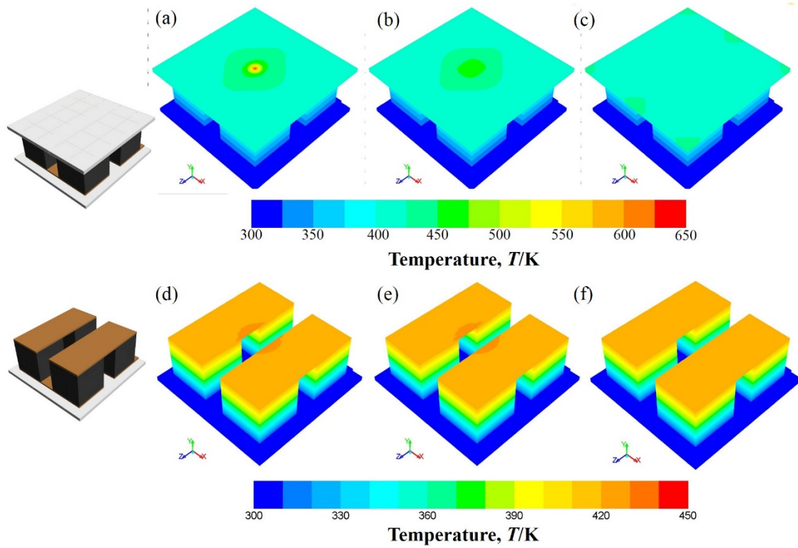
Fig.4 Temperature profiles on the surface of TE elements. (a)-(c): on the upper surface of alumina plate. (d)-(f): the alumina plate is removed. (a) and (d) are for Model I, (b) and (e) for Model II, and (f) and (c) for Model III.
