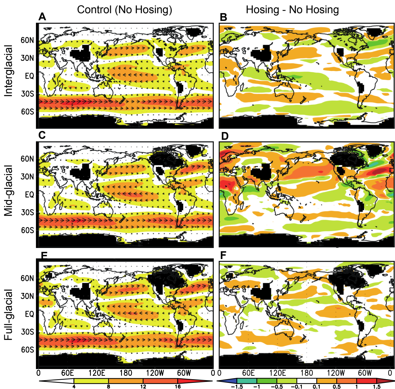
fig. S10. Results of MIROC climate model simulation of wind speed. (A) Wind speed at 850 hPa level for interglacial control run (without freshwater hosing). (B) Anomaly of wind speed associated with release of 0.05-Sv freshwater hosing (average of 400–500 model years). As (A) and (B), but for (C) and (D), mid-glacial case, and (E) and (F), full-glacial case, respectively.
