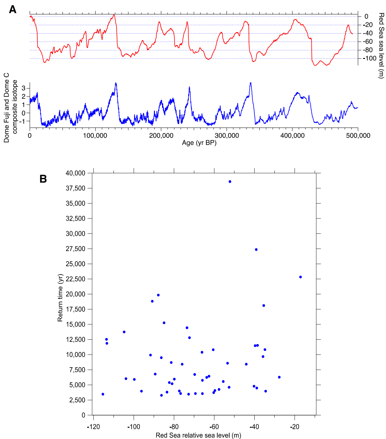
fig. S4. Return time of AIM compared with the Red Sea relative sea level. (A) Red Sea relative sea level (80) and Antarctic isotopic record (present study). (B) Return time of AIM with respect to sea level.
