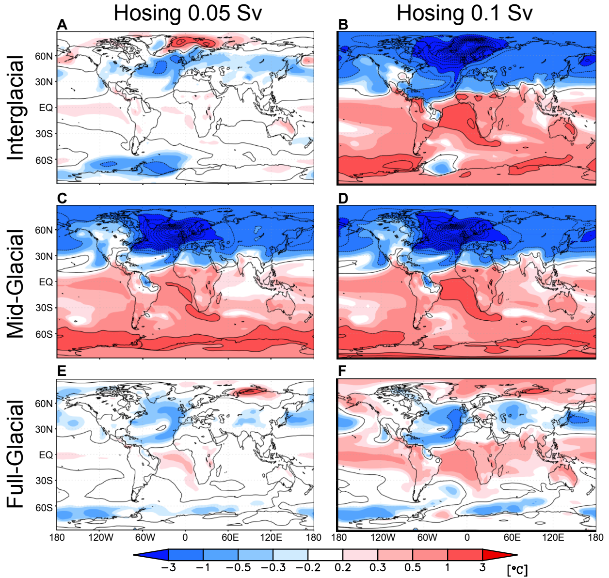
fig. S9. Simulation results with the MIROC climate model for surface air temperature change.
