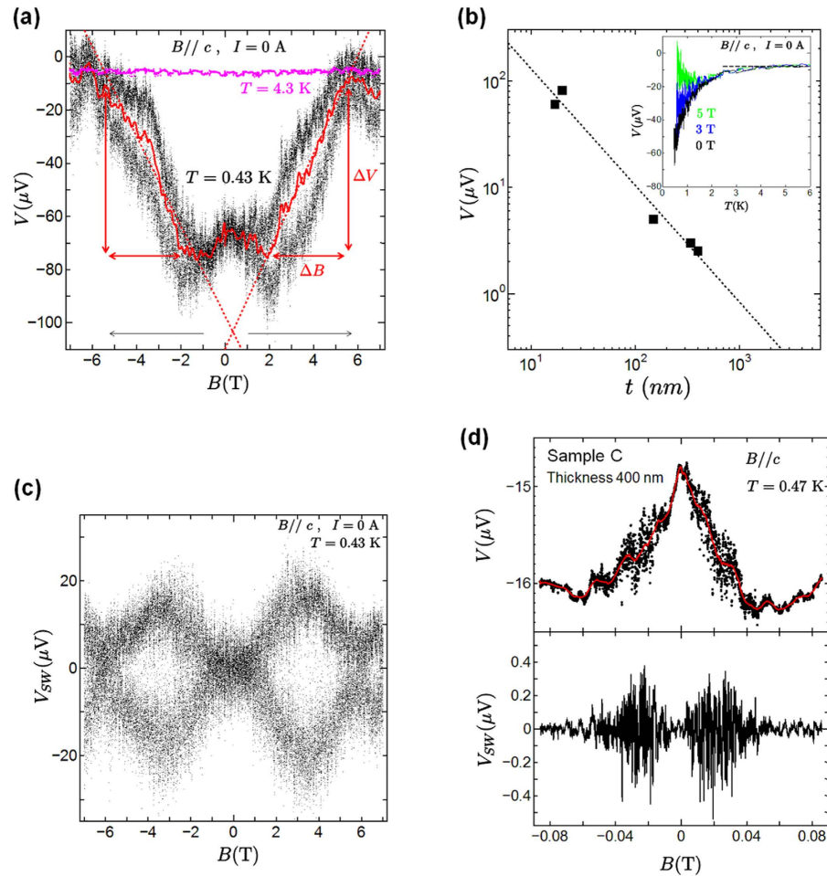
Figure 2. Topological magnetic-field-induced electric polarization. (a) Dependence of induced voltage on magnetic field at 0.43 and 4.3 K with zero bias current. Arrows represent the magnetic sweep direction from zero magnetic field to \pm 7 T. The solid red curve represents the average result for the measured data. (b) Thickness dependence of induced voltage at lower temperature. The dotted line represents the fitting result, which is described well by V = 1/t . The inset shows the temperature dependence of the induced voltage. (c) The anomalous switching voltage V_{SW} extracted from the B - V curves in (a). (d) Magnetic field dependence of V and V_{SW} for sample C.
