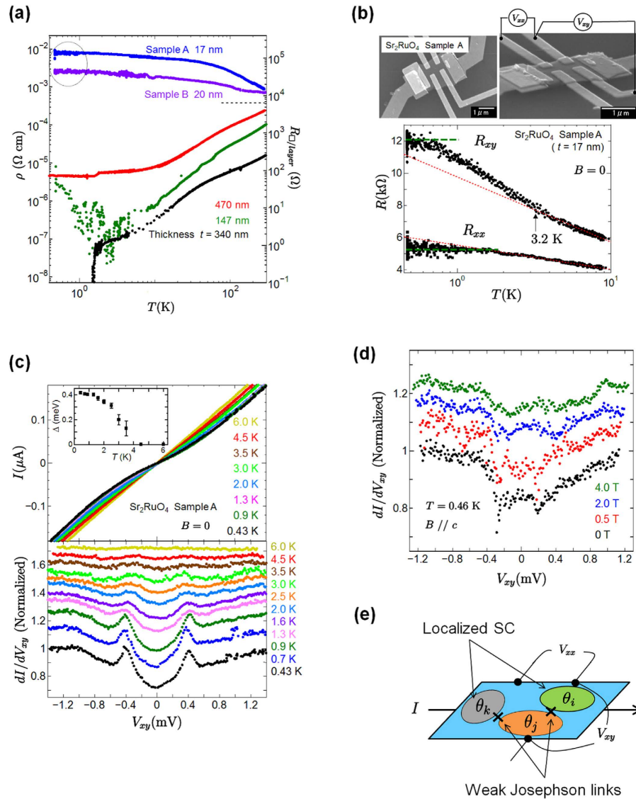
Figure 1. Superconductor-insulator transition driven by varying thickness and local superconductivity in \text{Sr}_2\text{RuO}_4 nanofilms. (a) Temperature dependence of the resistivity \rho_{xx} for different thicknesses of \text{Sr}_2\text{RuO}_4 single crystals. R_{\square}/\text{layer} is resistance per square per \text{RuO}_2 layer. The dotted horizontal line represents (h/4e^2) = 6.45 \text{ k}\Omega . (b) Scanning electron micrographs of the top and side views of sample A. Temperature dependence of R_{xy} and R_{xx} . The dotted horizontal lines are a guide for the eye. (c) V_{xy} - I characteristics for sample A at temperatures in a zero magnetic field. dI/dV_{xy} as a function of V_{xy} . The inset shows the temperature dependence of the superconducting gap \Delta . (d) Tunneling spectra dI/dV_{xy} for sample A in various magnetic fields. (e) Schematic of local superconducting islands weakly coupled by tunneling junctions, where \theta is the superconducting phase. This may be similar to small Josephson junction arrays.
