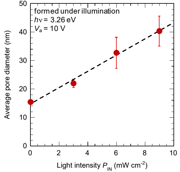
Fig. 5. Relationship between pore diameter and light intensity P_{IN} with h\nu = 3.26 eV.
