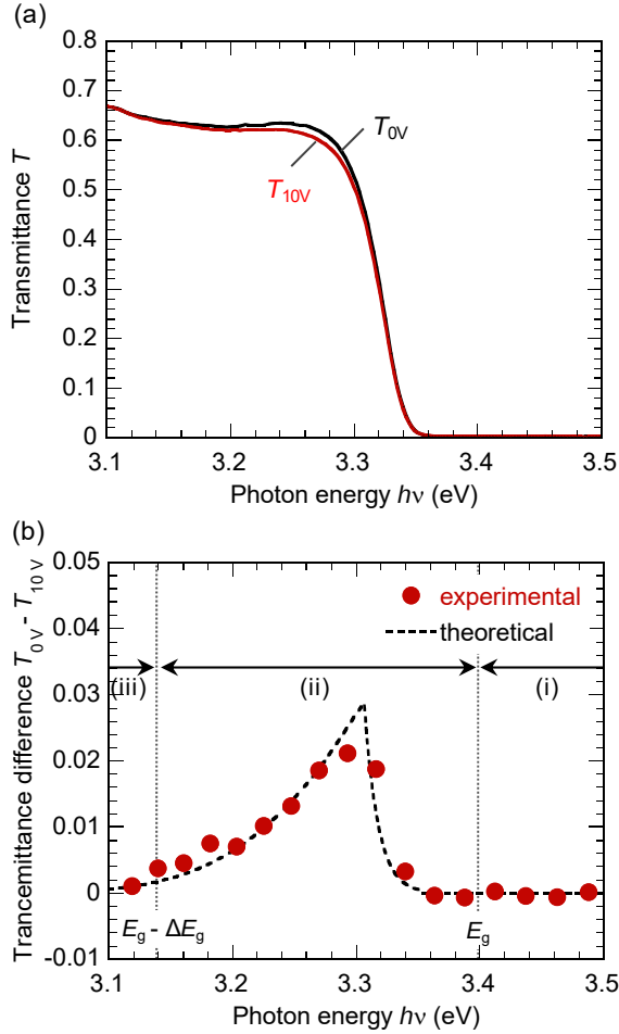
Fig. 6. (a) Transmittance spectra of a GaN planar electrode, obtained by applying anode voltages of V_a = 0 and 10 V in the electrochemical setup shown in Fig. 1. (b) Transmittance difference T_{0V} - T_{10V} plotted as a function of the photon energy h\nu .
