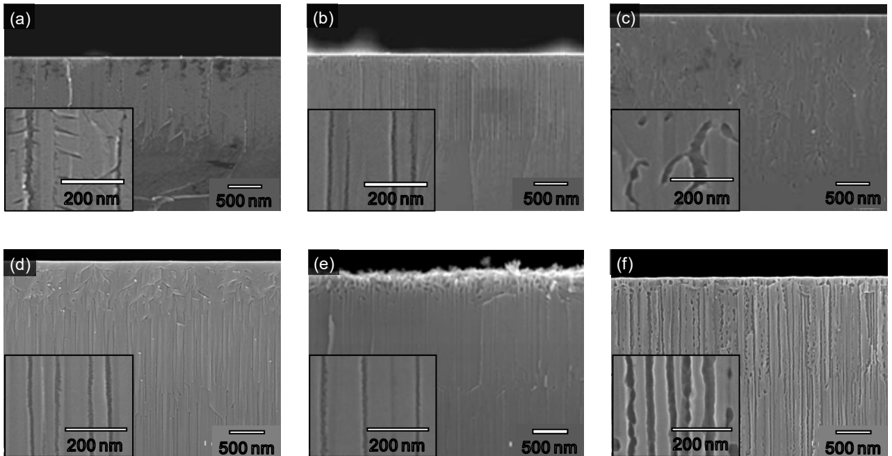
Fig. 3. Cross-sectional SEM images of GaN porous structures formed under various electrochemical conditions: (a) dark, t_a = 1200 s, V_a = 8 V; (b) dark, t_a = 1200 s, V_a = 10 V; (c) dark, t_a = 1200 s, V_a = 15 V; (d) dark, t_a = 2400 s, V_a = 10 V; (e) illuminated, t_a = 2400 s, V_a = 10 V, h\nu = 3.54 eV; (f) illuminated, t_a = 2400 s, V_a = 10 V, h\nu = 3.26 eV.
