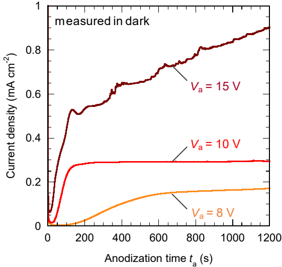
Fig. 2. Current-time curves obtained during anodization at various anode voltage V_a values.
