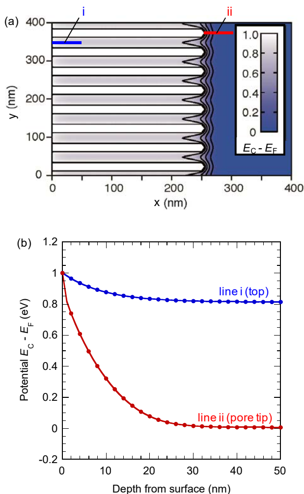
Fig. 7. (a) Potential distribution in GaN porous structures drawn with contour levels at 0.2, 0.4, 0.6, 0.8, and 1.0 eV, and (b) the cross-sectional potential distribution at the top surface (line i) and pore tips (line ii) obtained by solving 3D Poisson equation.
