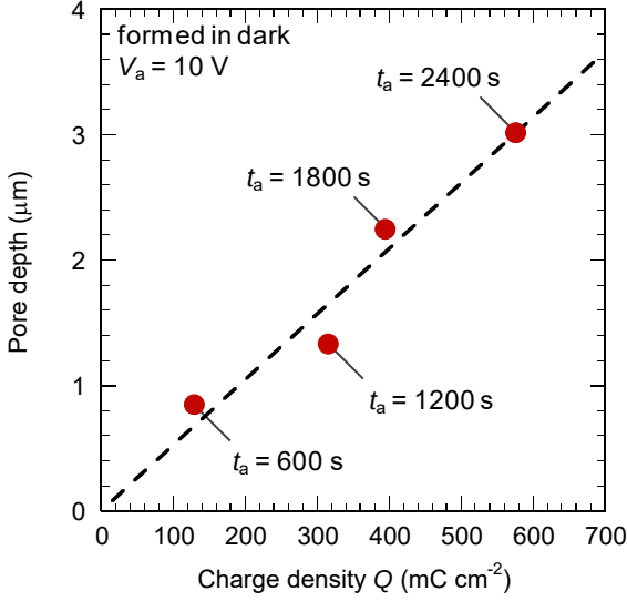
Fig. 4. Relationship between pore depth and density of charges, Q , passing through the working electrode during electrochemical etching.
