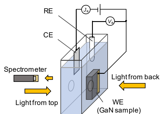
Fig. 1. Schematic illustration of the electrochemical setup used for both the formation of porous structures and the spectro-electrochemical measurements.
