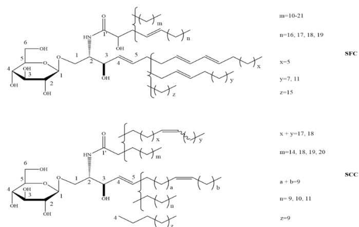
Fig. 1 The chemical structures of starfish cerebroside (SFC) and sea cucumber cerebroside (SCC).
