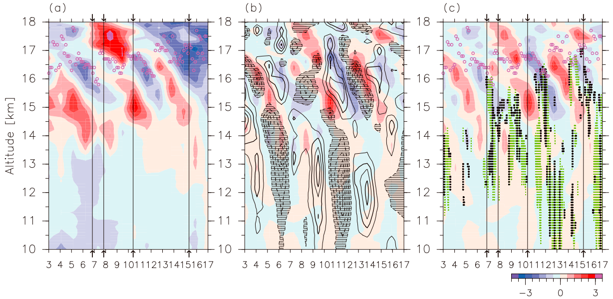
Figure 3. Time-altitude distributions of (a) temperature anomaly (colors; in K), (b) the <7 day filtered temperature (colors; in K) and velocity wind (contours and shading; 1.5 \text{ m s}^{-1} interval), and (c) temperature anomaly having <7 day periods (colors; in K) and the 1064 nm attenuated backscatter coefficient (green dots for all cirrus and black dots for SVC; regions with \geq 6.2 \times 10^{-5} \text{ km}^{-1} \text{ sr}^{-1} ) over the R/V Mirai at 10–18 km. The purple circles denote the location of the cold-point tropopause. Vertical lines denote the times of the CFH launches corresponding to results shown in Figure 2.
