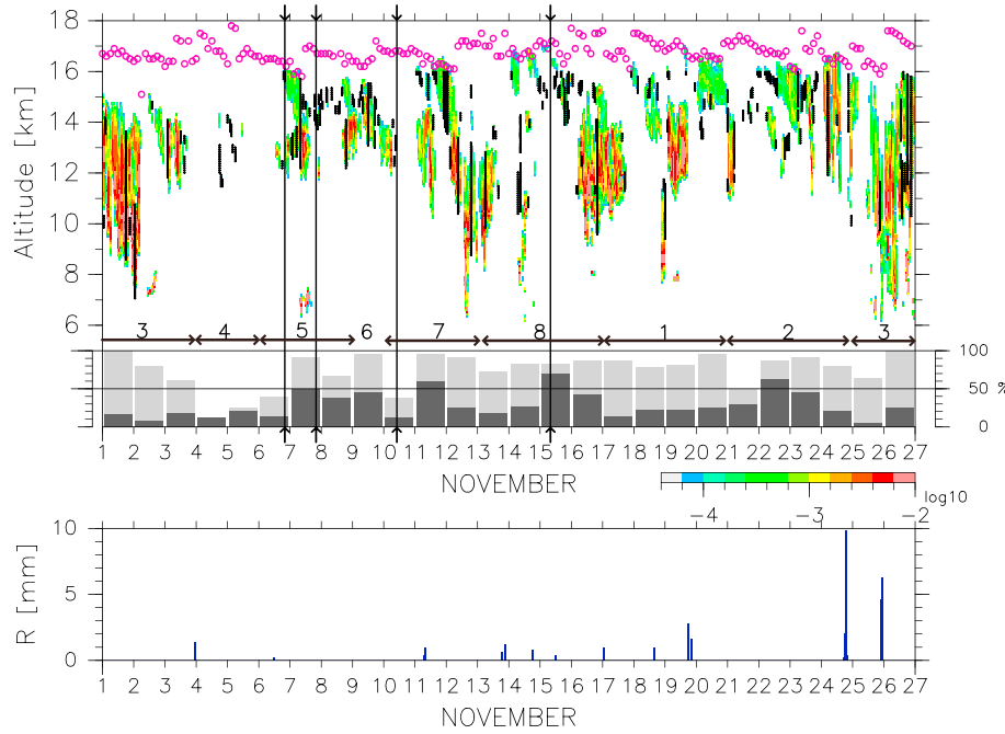
Figure 1. (top) Time-altitude distribution of the 1064 nm attenuated backscatter coefficient ( P_{1064} ) for the cirrus signals at 6–18 km over the R/V Mirai during the period of 1–26 November 2011. Regions with \geq 6.2 \times 10^{-5} \text{ km}^{-1} \text{ sr}^{-1} are colored. The location of SVC clouds ( \tau < 0.03 ) is indicated by black dots on the colored cloud signals. The purple circles denote the location of the cold-point tropopause. Gray-colored bars at the bottom indicate the cloud appearance frequency (%) for each day; darker bars are for SVC clouds only. The numbers (1–8) indicate the phase of the MJO index (see text for details). Vertical lines denote the times of the CFH launches corresponding to results shown in Figure 2. (bottom) Hourly surface rainfall at the R/V Mirai during the period of 1–26 November 2011.
