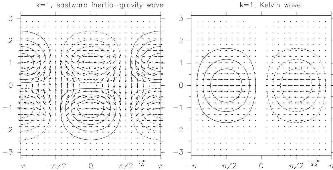
Figure 6. Horizontal structures of a nondimensional zonal wave number k=1 for theoretical solutions are shown for (left) n=0 eastward inertio-gravity equatorial waves and (right) equatorial Kelvin waves. Vectors denote the horizontal wind component. Contours show the geopotential at intervals of 0.25 arbitrary units. Negative contours are dashed, and the zero contour is omitted.
