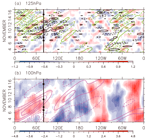
Figure 4. Longitude-time distributions at 7.5°S of (a) temperature anomaly of <7 day periods (colors; in K), n=0 eastward moving inertial gravity waves (black contours; 0.2 K interval) and equatorial Kelvin waves having <7 day period components (green contours; 0.2 K interval) at 125 hPa, and (b) temperature anomaly having >7 day periods (colors; in K) and the equatorial Kelvin wave component having >7 day periods (purple contours; 0.4 K interval) at 100 hPa. The wave extraction method is described in the text. The black lines indicate the location of the R/V Mirai , and the large black dots denote the times of the CFH launches corresponding to the results shown in Figure 2.
