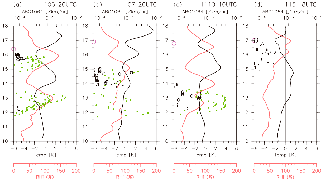
Figure 2. Profiles of temperature anomaly (black lines; in K), relative humidity over ice (red lines; %), and the 1064 nm attenuated backscatter coefficient (green circles for all cirrus and black circles for SVC ( \tau < 0.03 ); circles at \pm 4 h centered at the time of the CFH launch and larger circles at \pm 1 h of the CFH launch time in \text{km}^{-1} \text{ sr}^{-1} ) at 10–18 km on (a) 20 UTC in 6 November, (b) 20 UTC in 7 November, (c) 10 UTC in 10 November, and (d) 8 UTC in 15 November. The purple circles denote the location of the cold-point tropopause.
