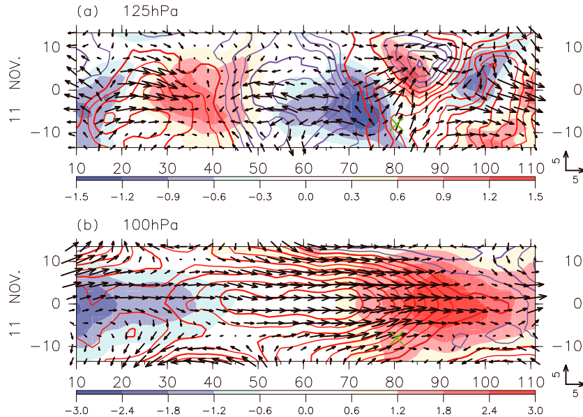
Figure 5. Longitude-latitude distributions of temperature (colors; in K), geopotential height (contours; 1.5 m interval), and horizontal wind components (vectors; \text{m s}^{-1} ) of (a) a <7 day period and (b) a >7 day period eastward propagating wave in 11 November. Green crosses indicate the location of the R/V Mirai (8.0°S, 80.5°E).
