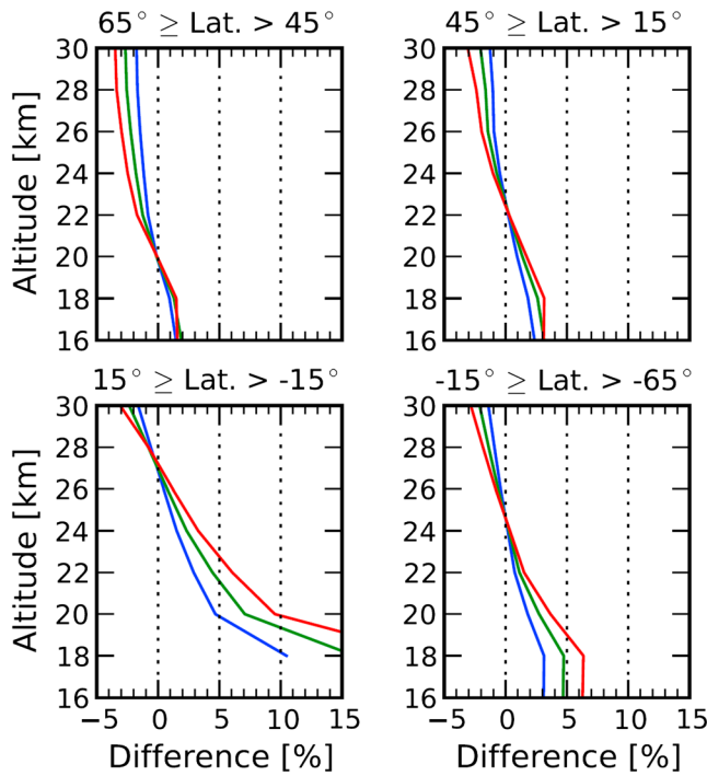
Figure 10. Correction amount to original mixing ratios averaged over the all ozonesonde profiles for the four latitude bands, 65°N–45°N, 45°N–15°N, 15°N–15°S, and 15°S–65°S with response times of 20 s (blue), 25 s (green), and 30 s (red).
