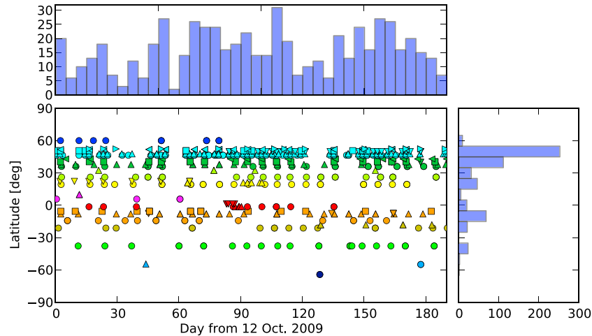
Figure 3. (bottom left) Temporal and latitudinal distribution of the coinciding ozonesonde measurements and the number of observations (top) for each 5 day period and (bottom right) for every 10° latitude bins. The symbols and the color in Figure 3 (bottom left) are the same as those in Figure 2.
