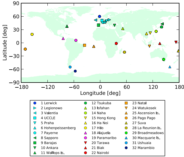
Figure 2. Global distribution of ozonesonde observation sites. The symbols for the sites are color coded in each 10° latitude bin. The number in the legend corresponds to the site number in Table 1.
