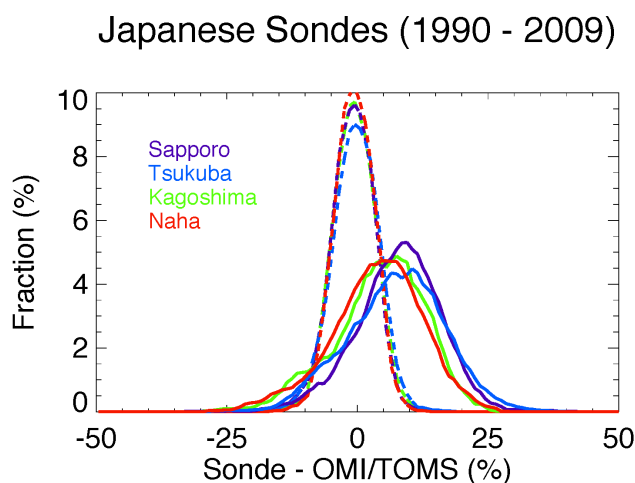
Fig. 1. A comparison of column ozone between integrated ozonesonde profiles from and the TOMS/OMI overpass data for the four Japanese stations. The thick lines represent data without the CF, while the dashed lines represent the data multiplied by the correction factor (CF) as applied and cited in the WOUDC data files. Kagoshima data cease in 2005.
