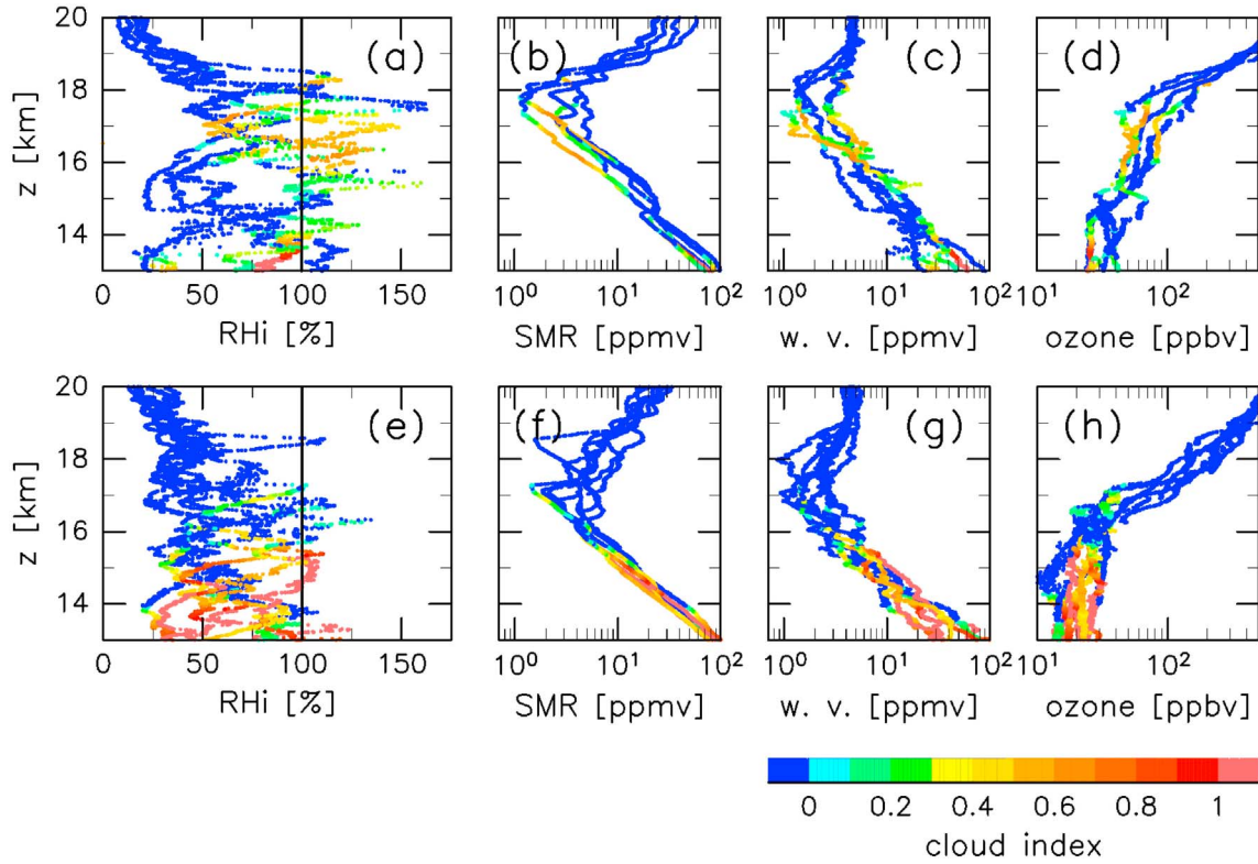
Figure 2. Vertical profiles of (a, e) RH i , (b, f) saturation water vapor mixing ratio, (c, g) water vapor mixing ratio, and (d, h) ozone mixing ratio for all the collocated measurements at Kototabang (Figures 2a–2d) and at Biak (Figures 2e–2h). The color shows the 10-base logarithm of backscattering ratio to the cloud threshold value (i.e., the cloud index defined by Equation (3)) calculated from CALIOP data.
