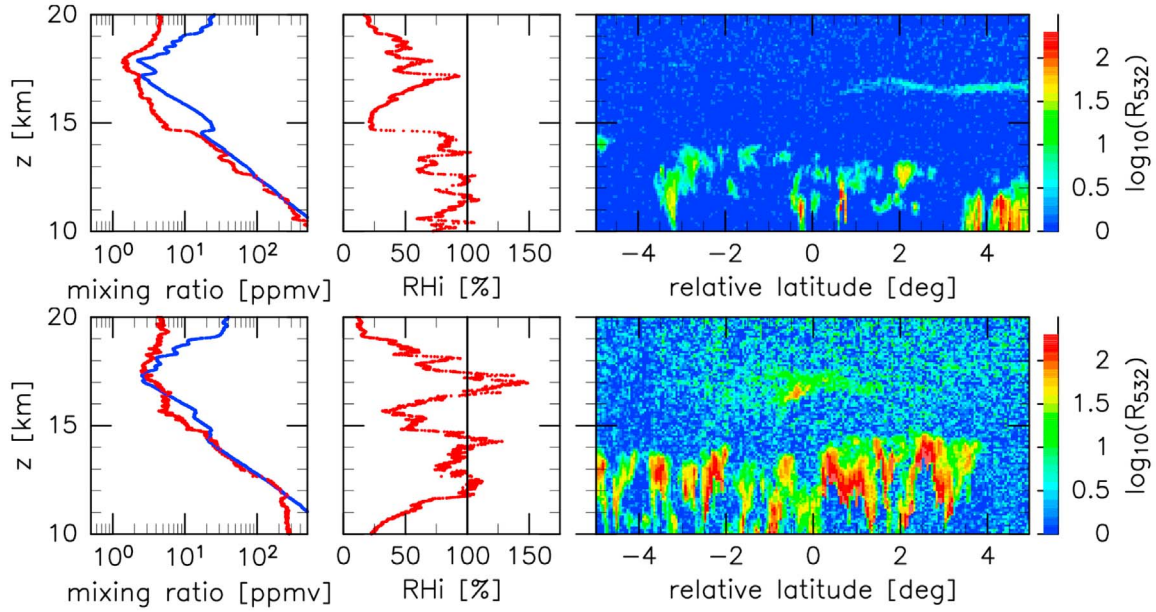
Figure 1. Examples of collocated measurements (top) at Kototabang on January 9, 2008 (23:59 UTC for CFH and 19:18 UTC at 0° relative latitude for CALIOP; the longitude difference between the two measurements is 3.92°) and (bottom) at Kototabang on January 11, 2007 (01:42 UTC for CFH and 07:15 UTC at 0° relative latitude for CALIOP; the longitude difference between the two measurements is 3.02°). (left) Vertical profiles of saturation water vapor mixing ratio (blue) and water vapor mixing ratio (red). (middle) Relative humidity over ice (red). (right) Latitude-altitude distribution of backscattering ratio R_{532} (color) along the CALIOP track (the latitude is relative to the CFH launch site).
