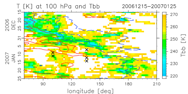
Figure 3. Longitude-time distributions of temperature anomaly at 100 hPa with respect to 191 K (contours with their interval 2 K: red solid lines (positive) and blue dashed lines (negative)) and equivalent black body temperature (T bb ) (colors) during the period from December 15, 2006 to January 25, 2007. Crosses indicate the sonde measurements.
